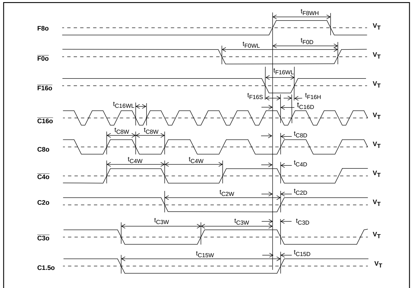
Figure 12 - Output Timing 1
