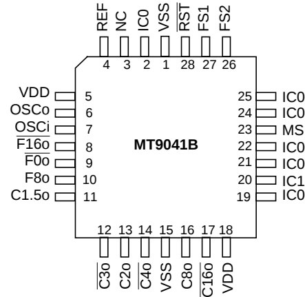
Figure 2 - Pin Connections
