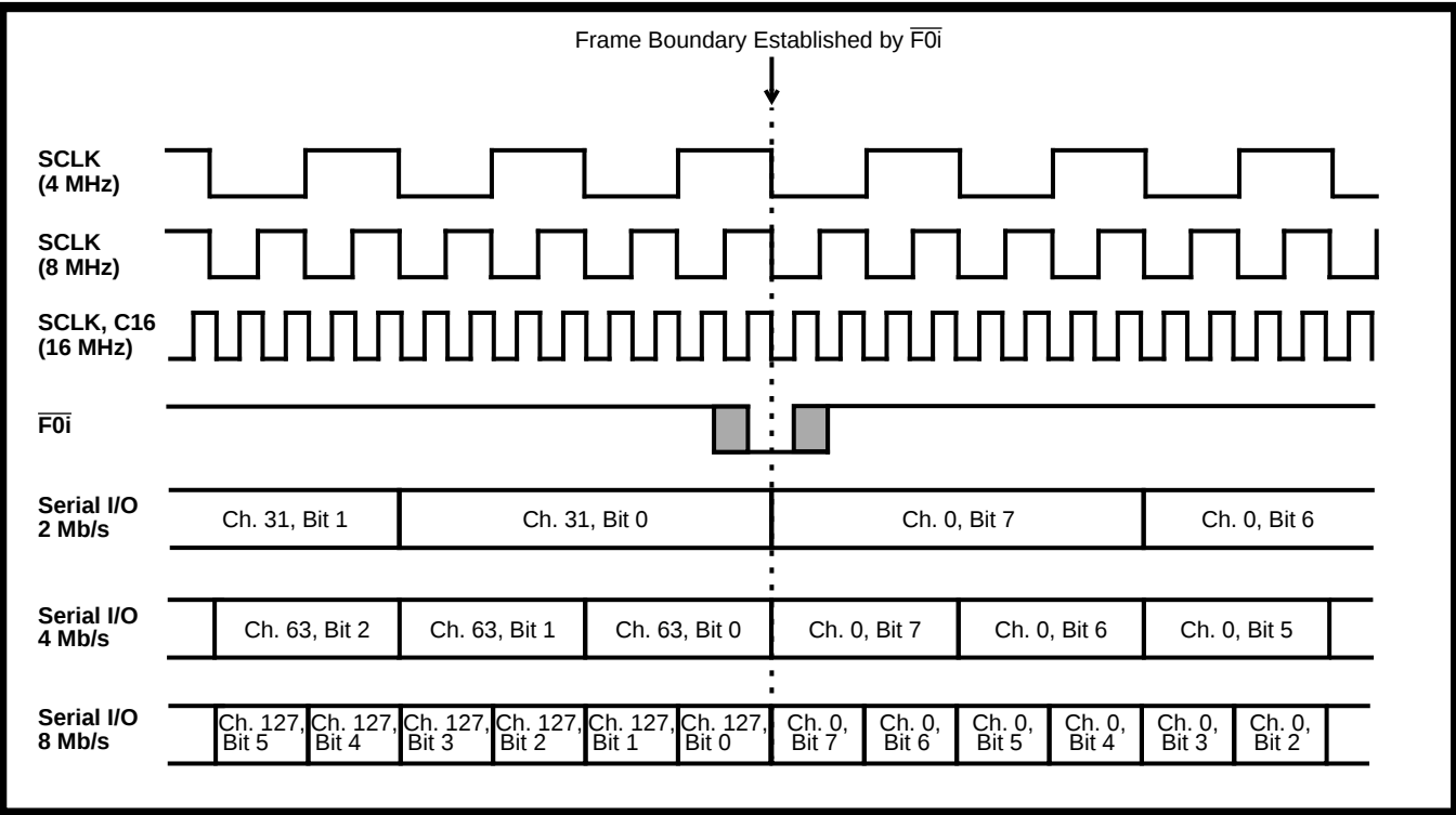
Figure 6 - Serial Port Functional Timing
