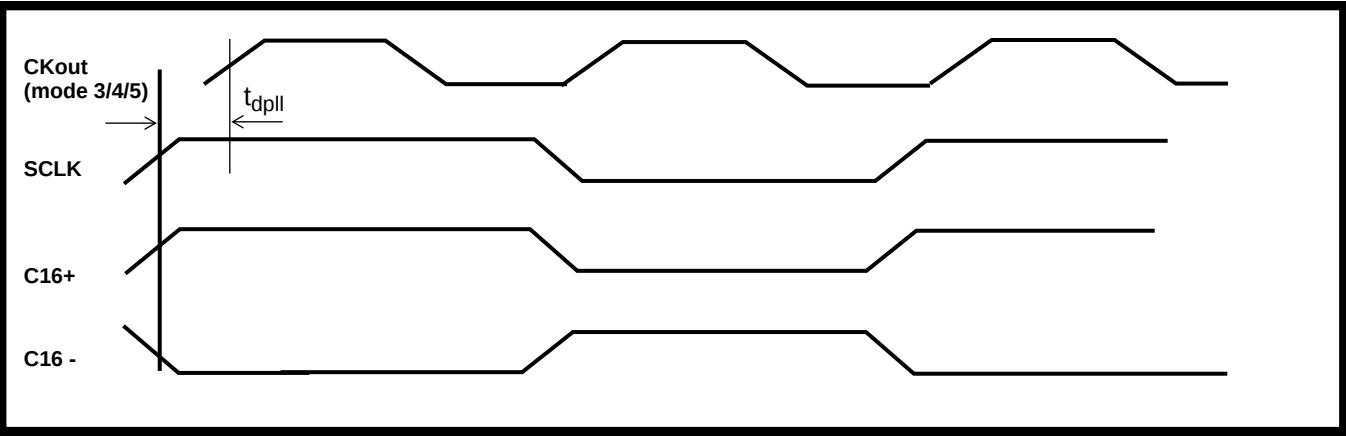
Figure 21 - PLL Timing
