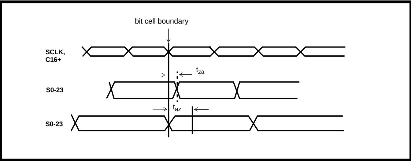
Figure 20 - Serial Port Tri-state Timing
