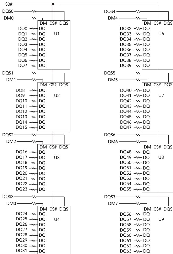
Figure 3: Functional Block Diagram – Standard PCB
