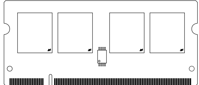
Figure 1: 200-Pin SODIMM (MO-224 R/C B)
