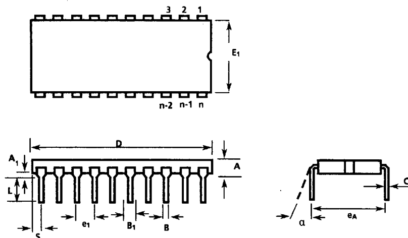
Ceramic Dual-In-Line Packages (CDIP) - C Suffix
