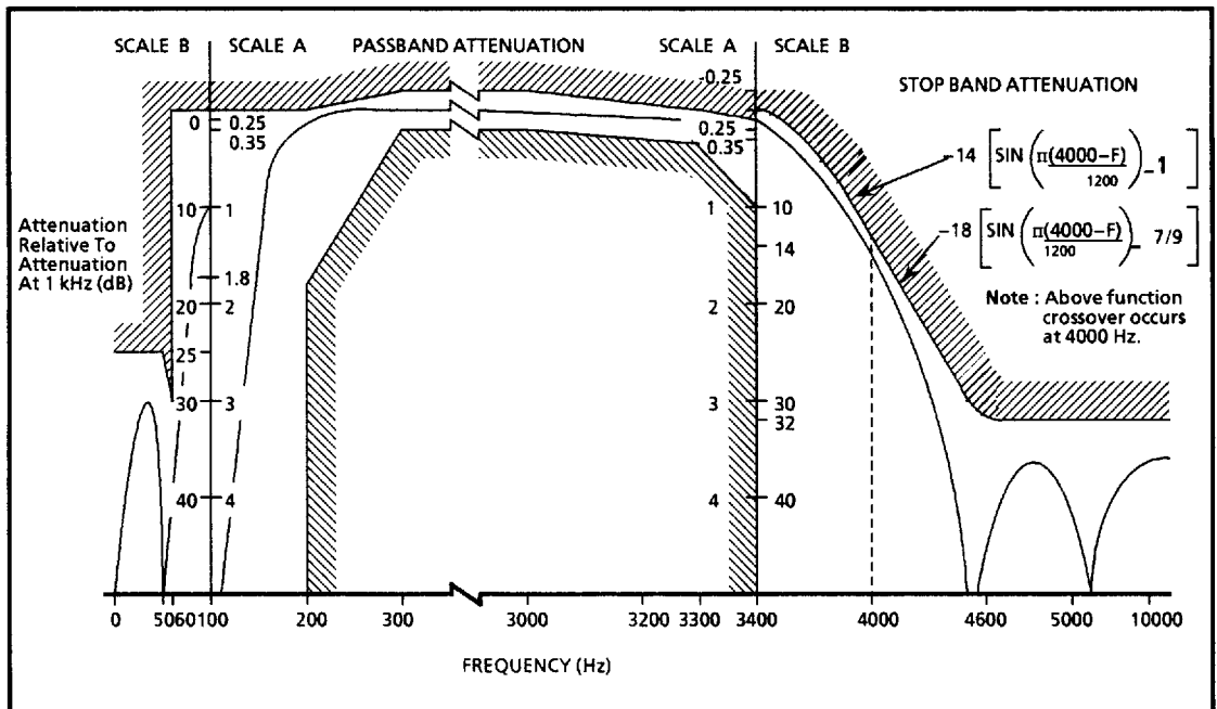
Figure 18 - Attenuation vs Frequency for Transmit Filter
