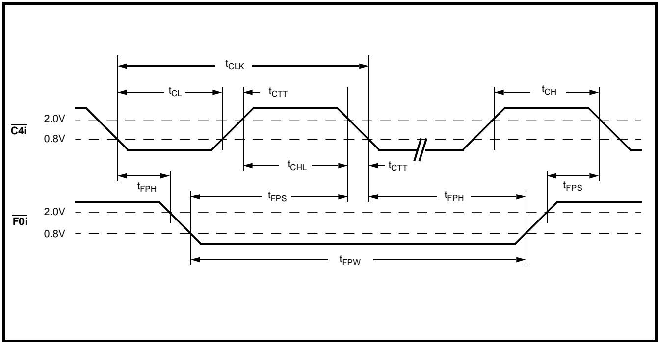
Figure 13 - Clock Timing
