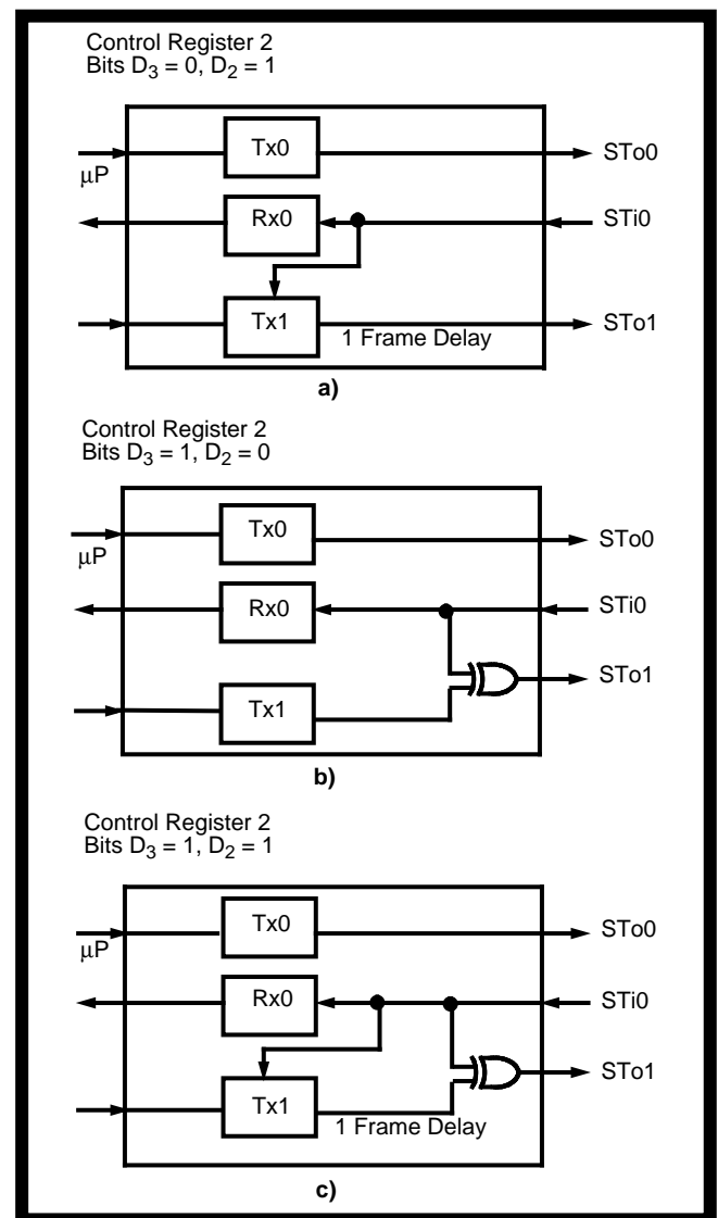
Figure 6 - ST01 Configurations
