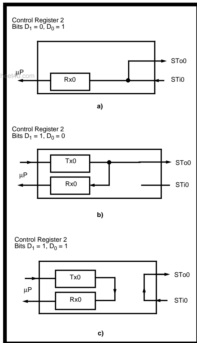
Figure 5 - Loopback Configurations
