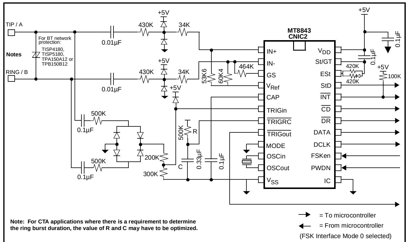
Figure 9 - Application Circuit
