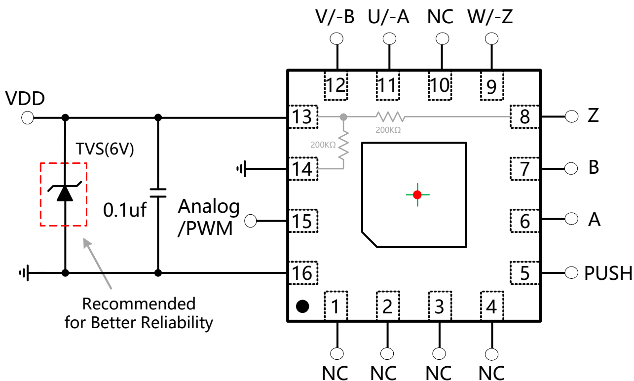
Figure 7: MT6701QT(QFN-16) Reference Circuit for ABZ/UVW/PWM/Analog/Push Output
