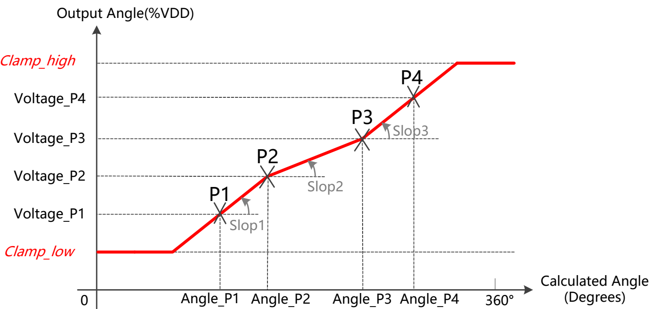
Figure 11: 4-Points Programmable Output Transfer Function
