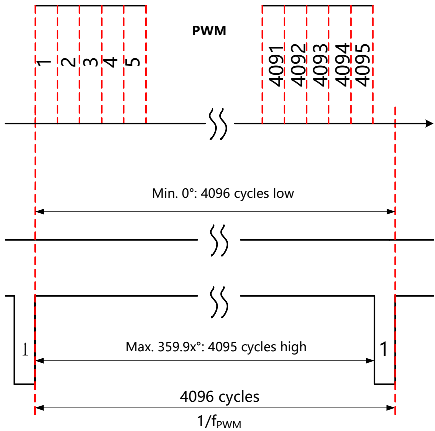
Figure 7: PWM Output
