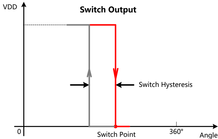
Figure 8: Switch Output
