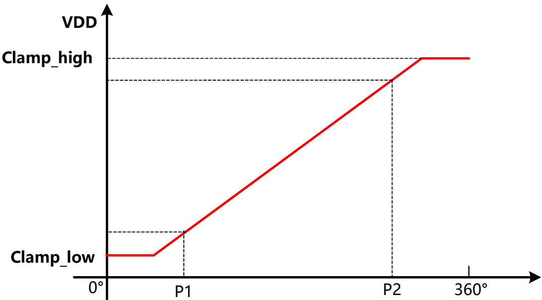
Figure 6: Analog Output
