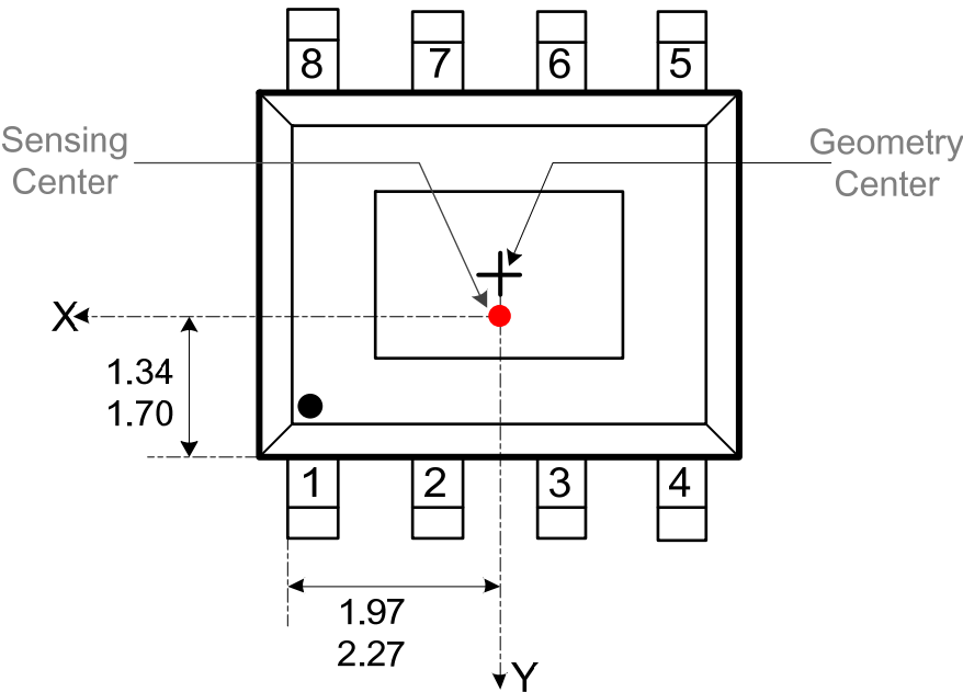
Figure 1: Pin Configuration for SOP-8 Package
