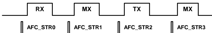
Figure 51 Timing Diagram for the AFC Controller
