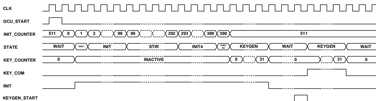
Figure 33 The timing diagram of the GCU (in case of GEA2)
