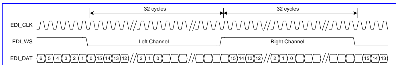
Figure 64 Cycle count is 32 for I2S format.
