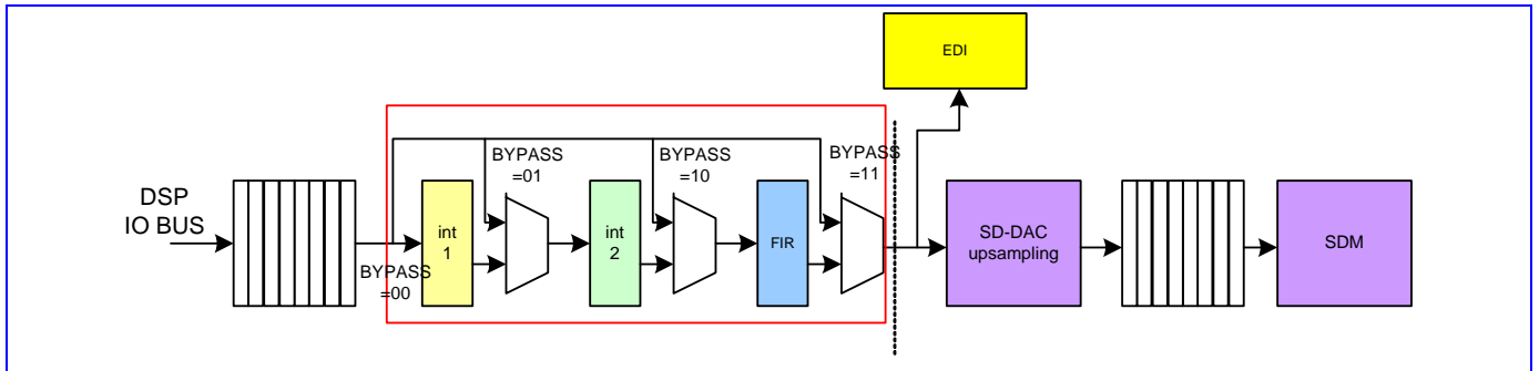
Figure 62 Block diagram of the audio path.
