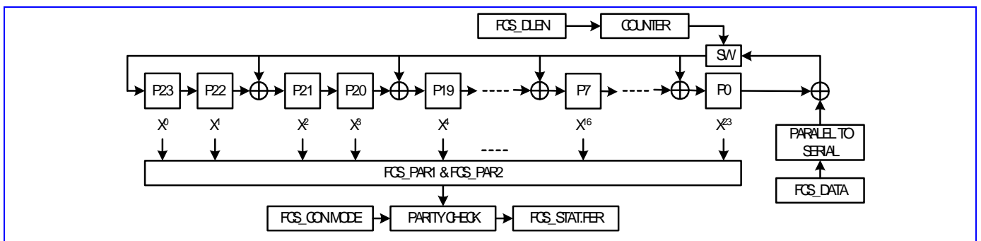
Figure 42 FCS codec circuit.
