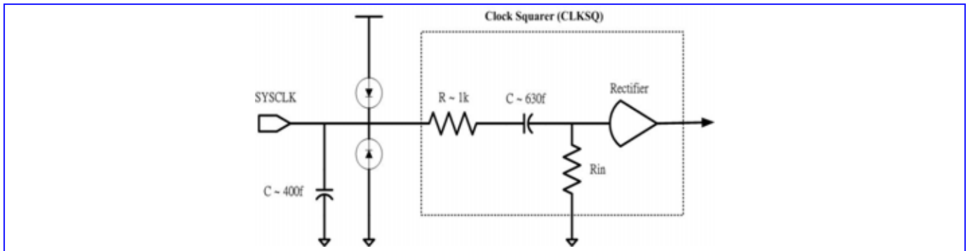
Figure 76 Equivalent circuit of Clock Squarer.
