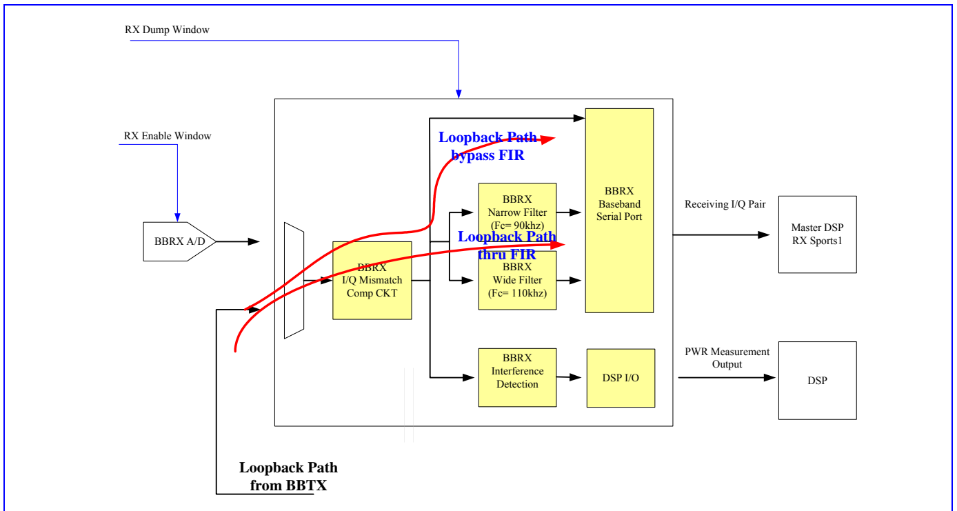
Figure 53 Block diagram of RX path
