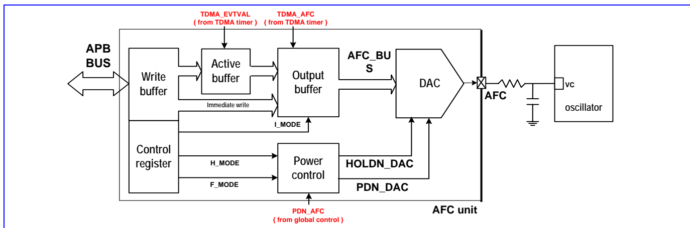
Figure 50 The block diagram of the AFC controller
