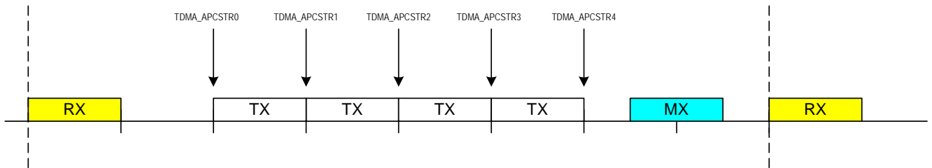
Figure 47 Timing diagram of TDMA_APCSTR.
