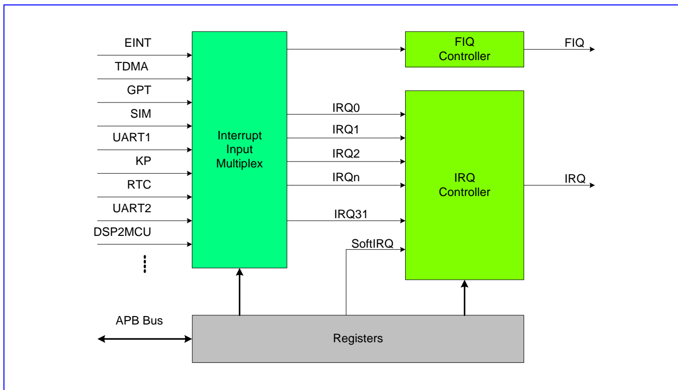
Figure 14 Block Diagram of the Interrupt Controller
