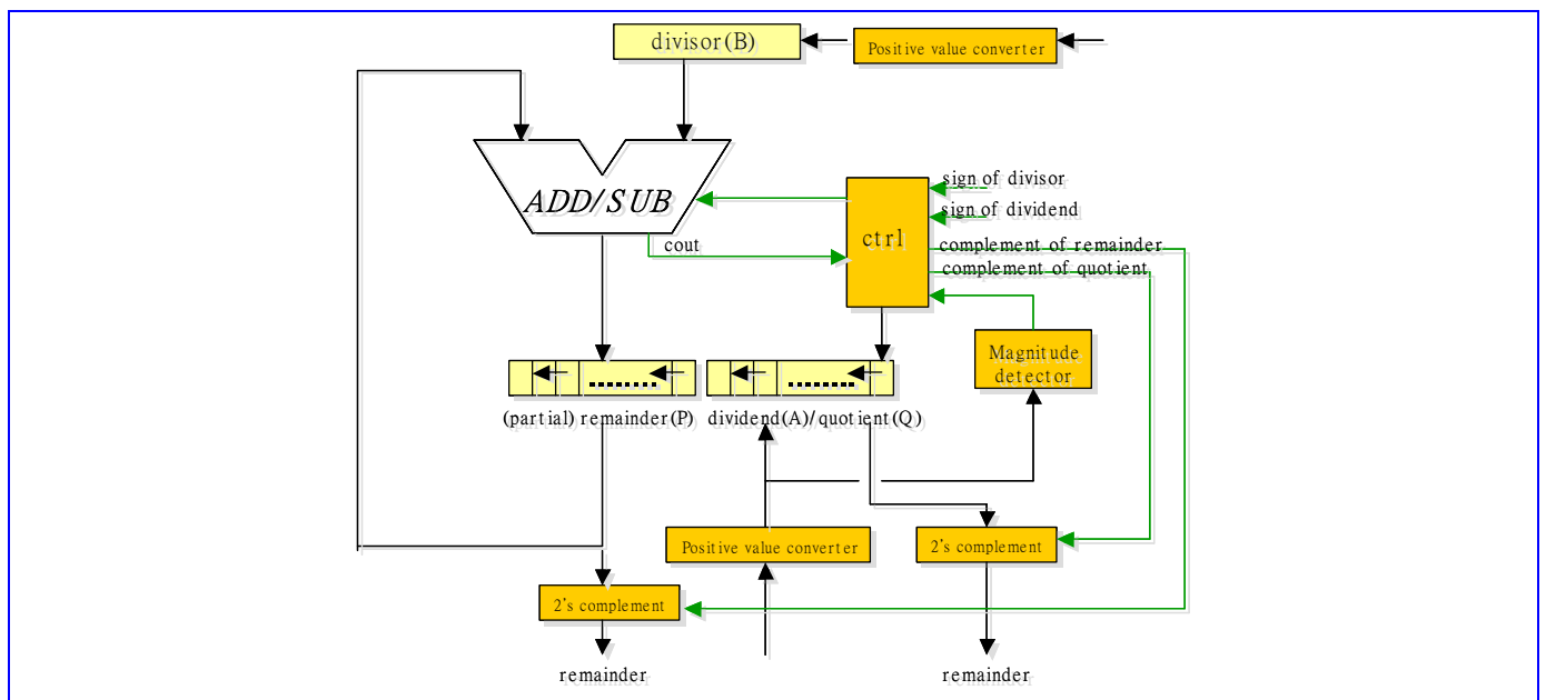
Figure 35 Architecture of radix-2 non-restoring divider for MCU system
