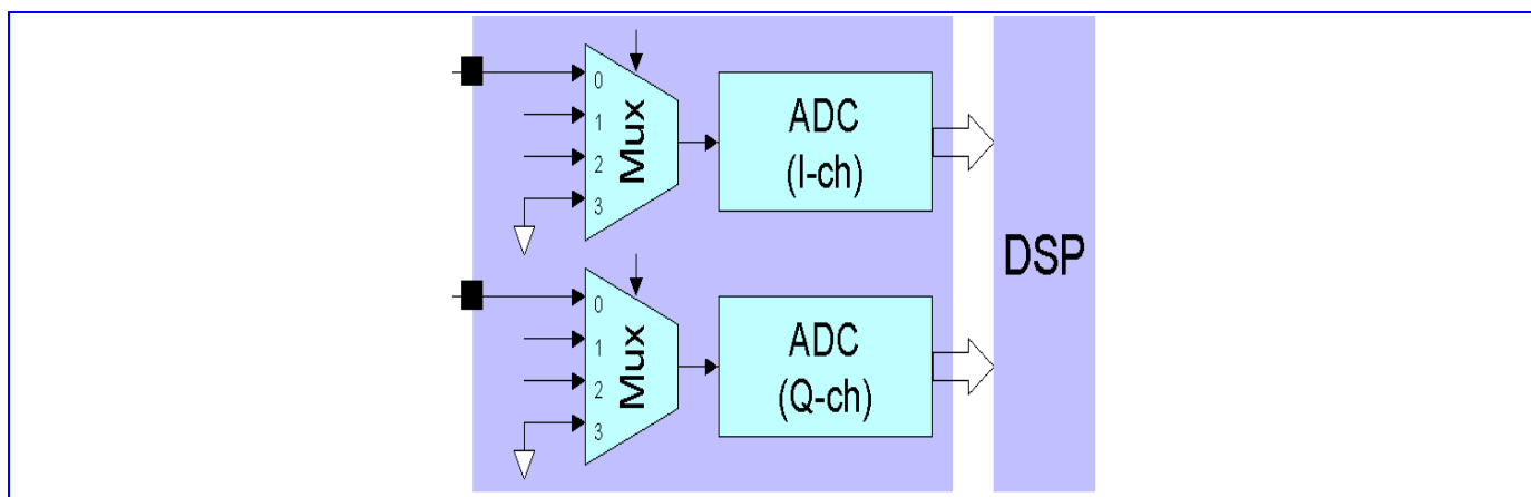
Figure 79 Downlink ADC Offset Error Measurement
