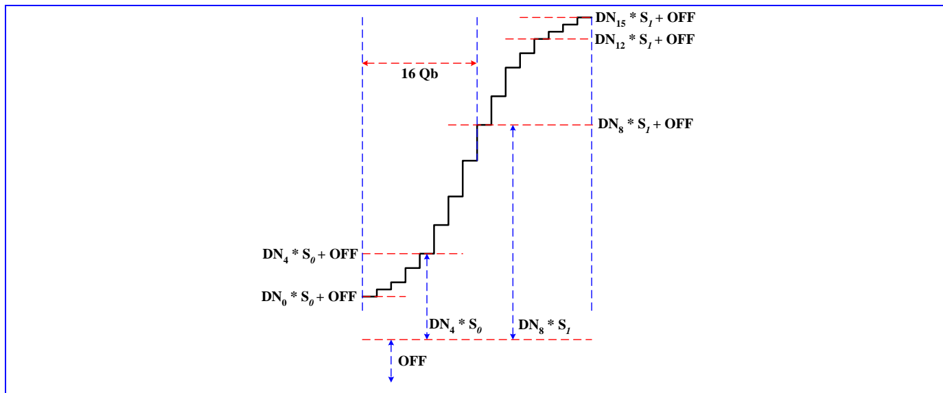
Figure 48 The timing diagram of the APC ramp.
