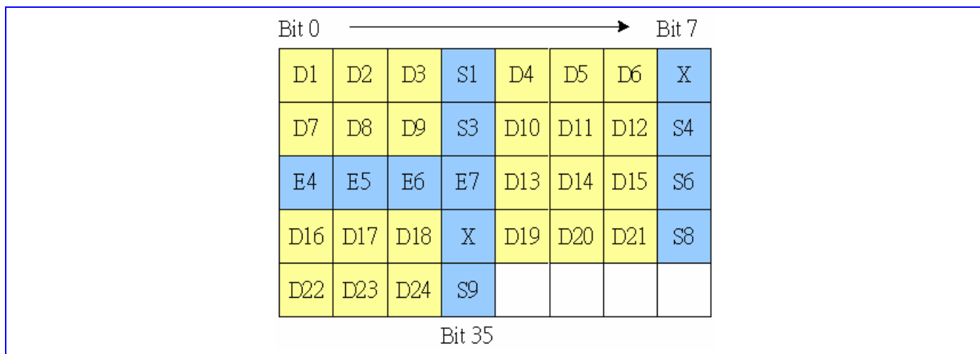
Figure 38 data format conversion for 3.6k RA1
