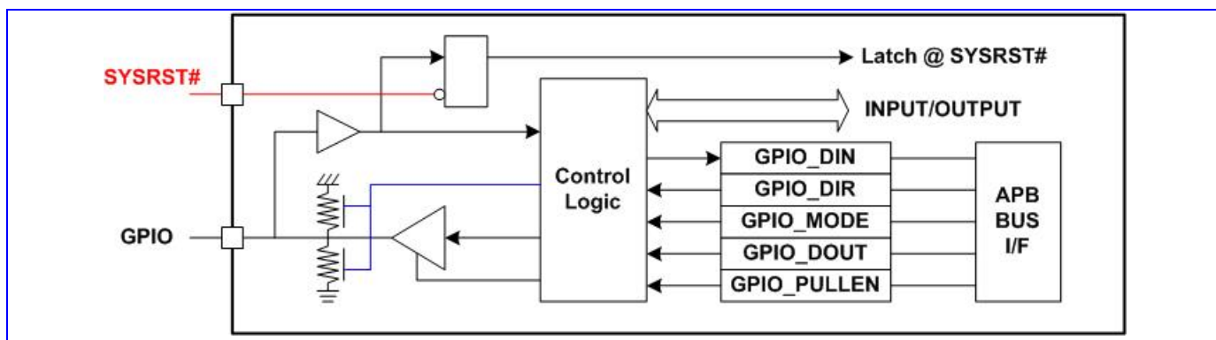
Figure 30 GPIO Block Diagram
