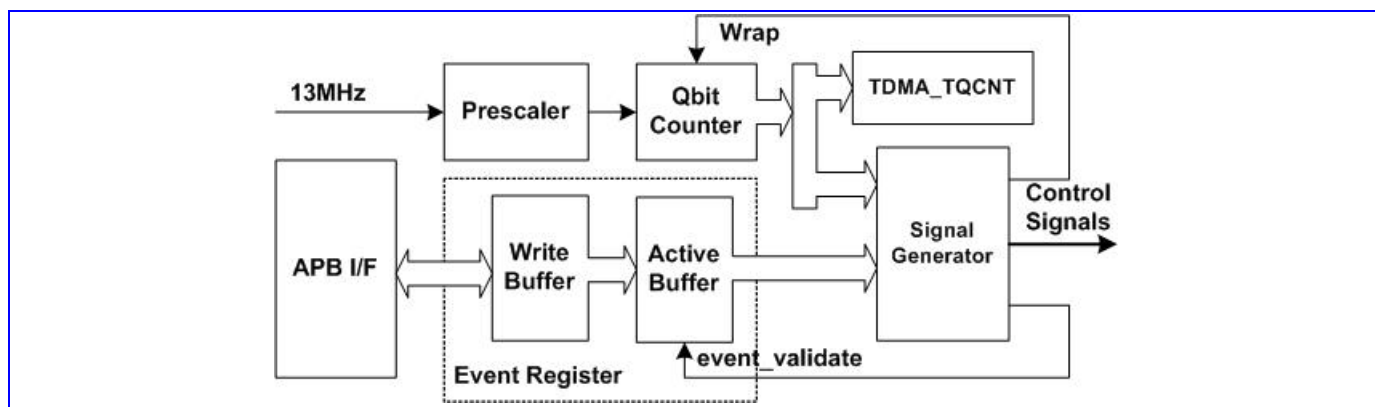
Figure 65 The block diagram of TDMA timer
