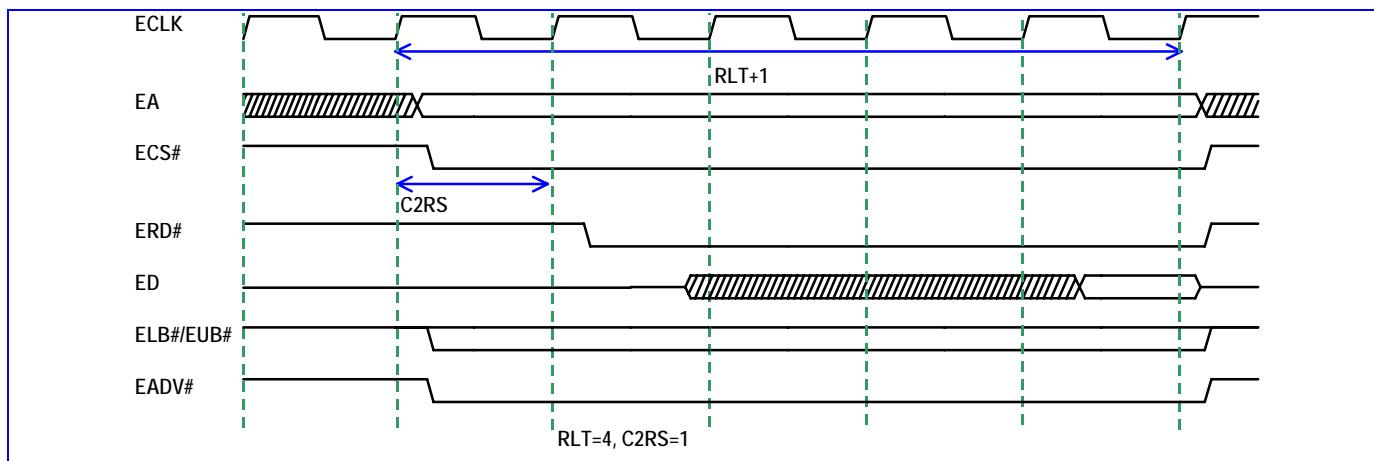
Figure 16 Read Wait State Timing Diagram (ADVR=1)
