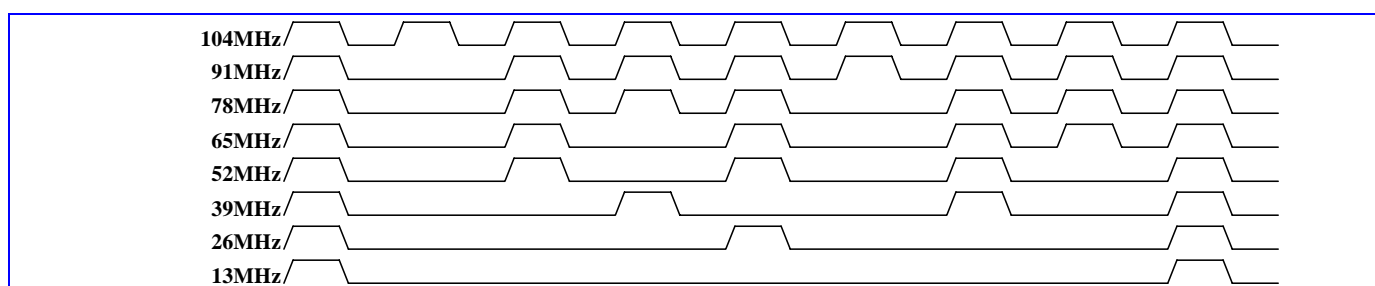
Figure 72 Output of Dynamic Clock Manager
