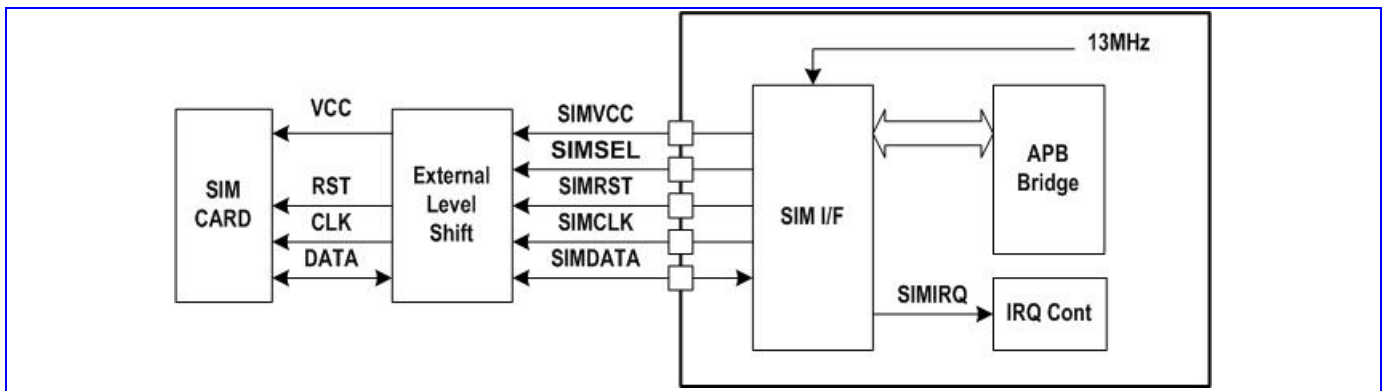
Figure 23 SIM Interface Block Diagram
