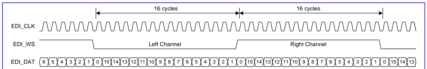
Figure 63 Cycle count is 16 for I2S format.
