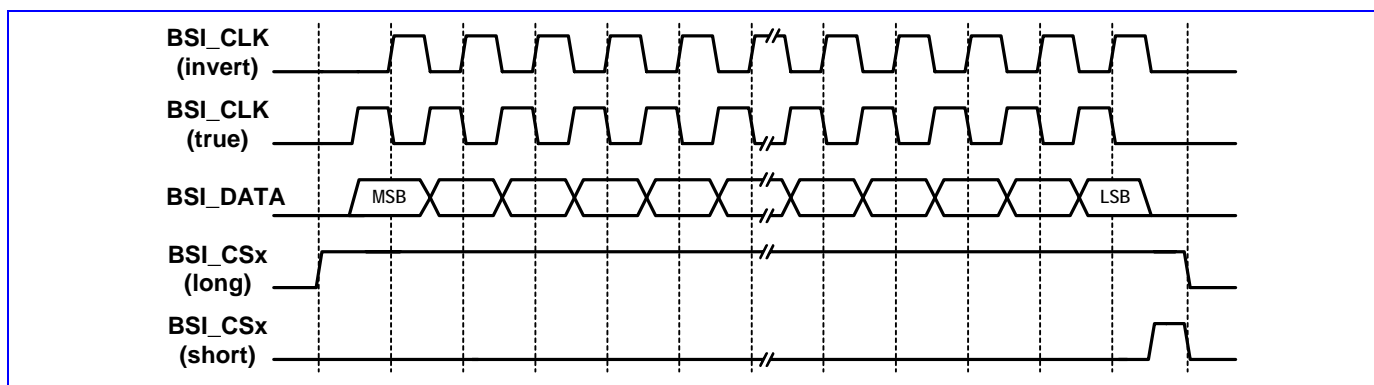
Figure 44 Timing characteristic of BSI interface.
