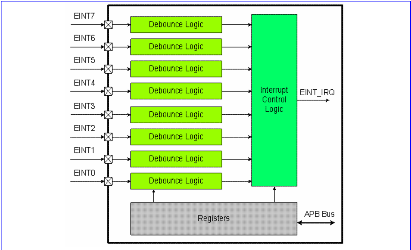
Figure 15 Block diagram of External Interrupt Controller
