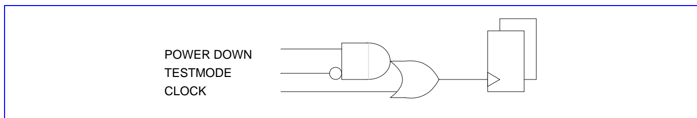
Figure 69 Power Down Control at Block Level
