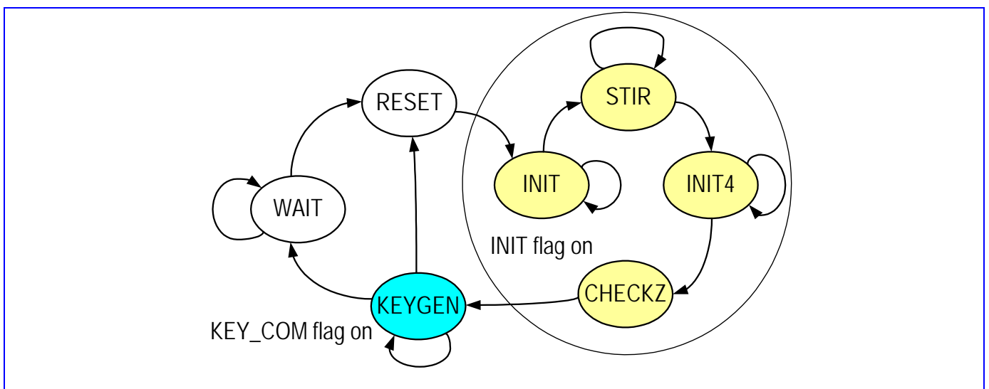
Figure 32 The state diagram of the GCU
