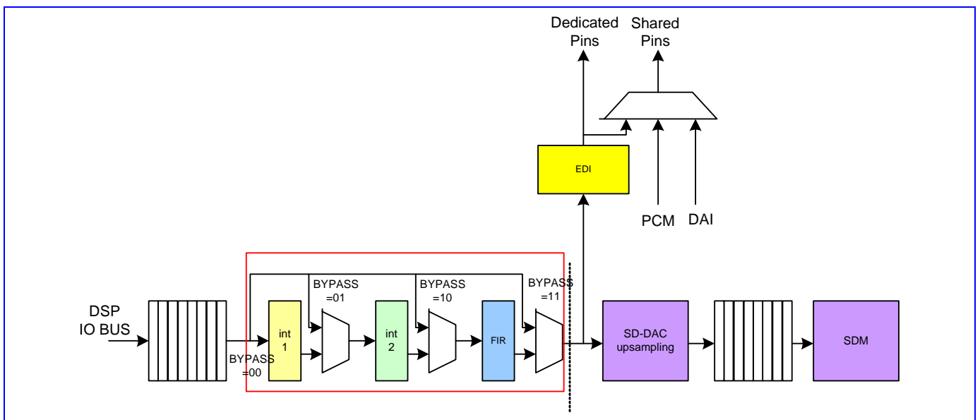
Figure 61 DAI, PCM, EDI interfaces
