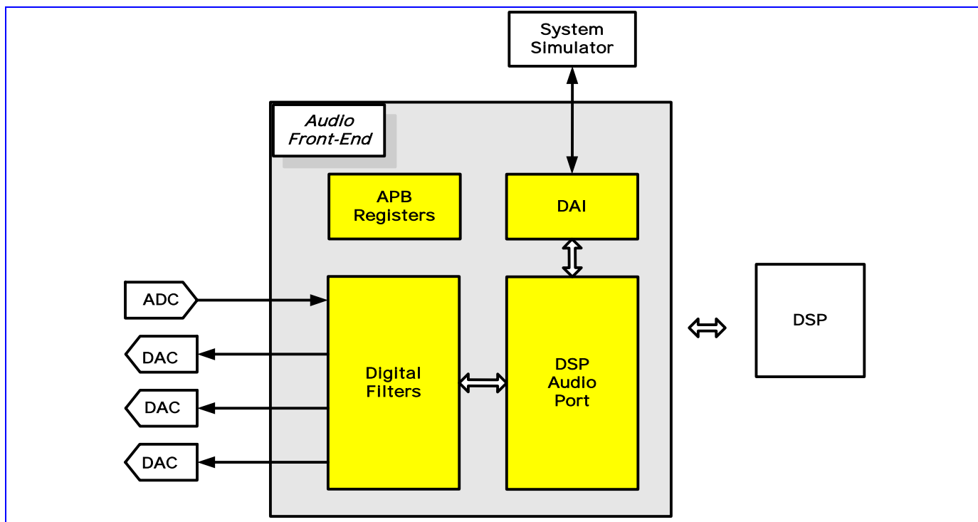
Figure 57 Block diagram of digital circuits of the audio front-end
