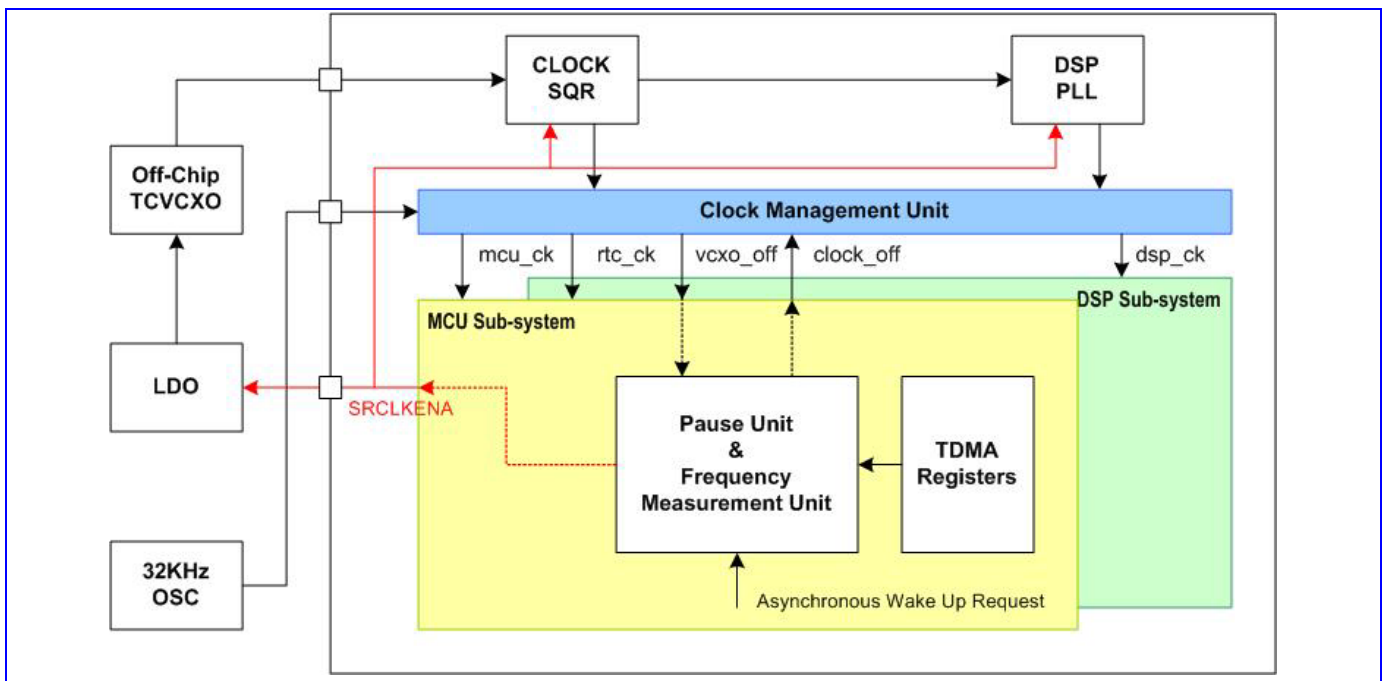
Figure 68 The block diagram of the slow clocking unit
