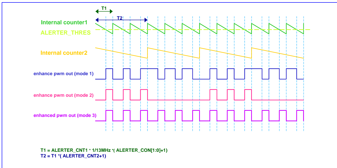
Figure 21 Alerter Waveform
