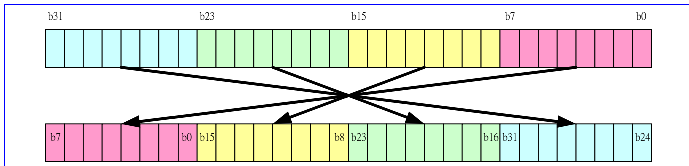
Figure 40 Type 2 bit reverse
