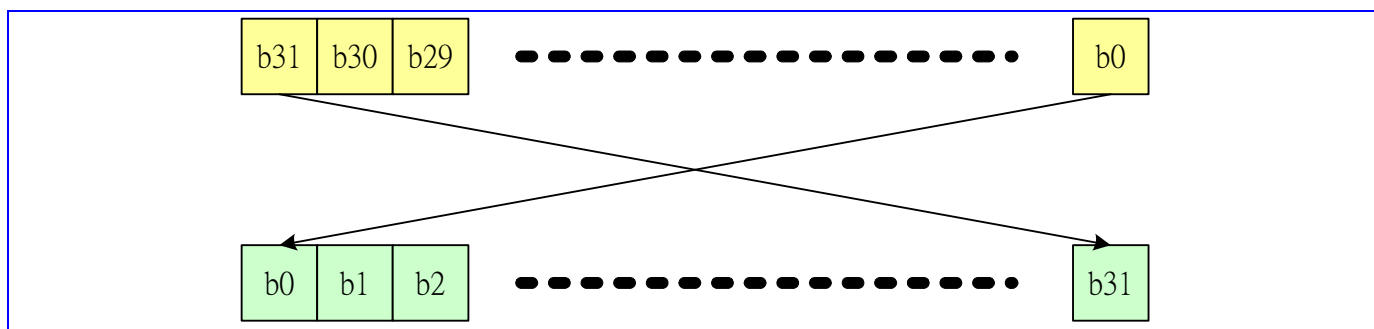
Figure 39 Type 1 bit reverse
