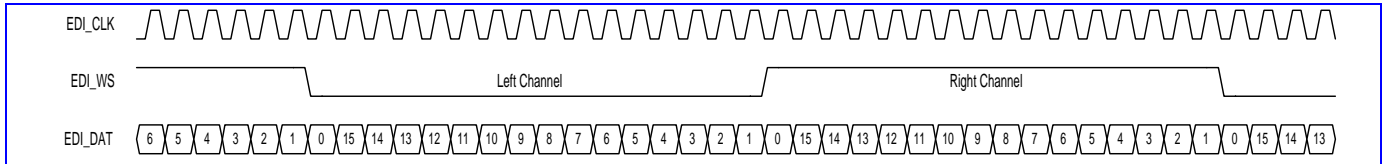
Figure 60 EDI Format 2: I²S (FMT = 1).
