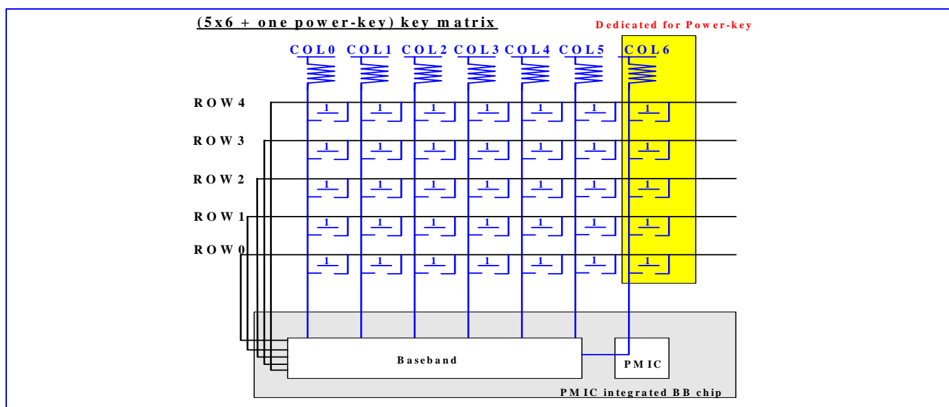
Fig. 1 5x6 matrix with one power-key
