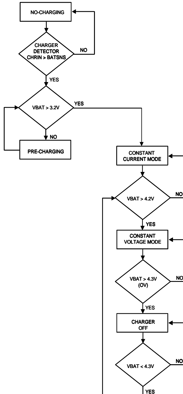
Figure 2. Battery Charger Flow Chart
