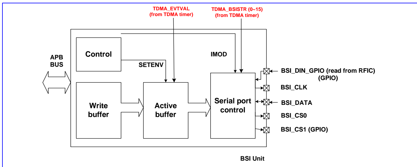
Figure 43 Block diagram of BSI unit.
