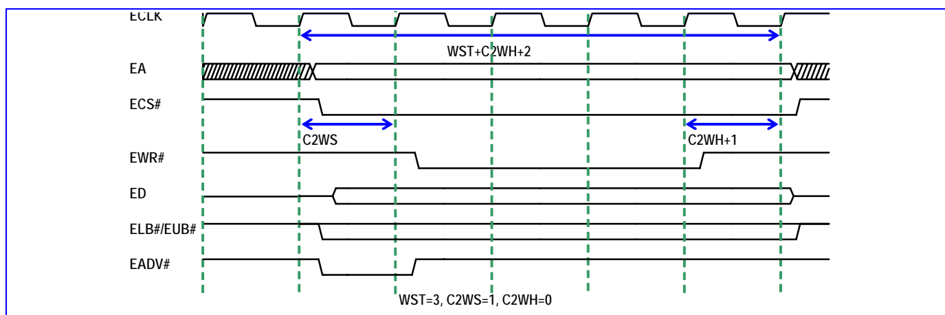
Figure 19 Write Wait State Timing Diagram (ADVW=0)
