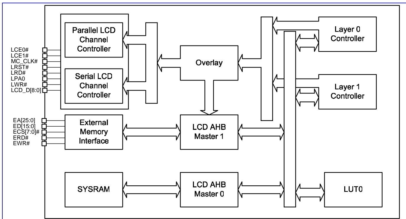
Figure 26 LCD Interface Block Diagram
