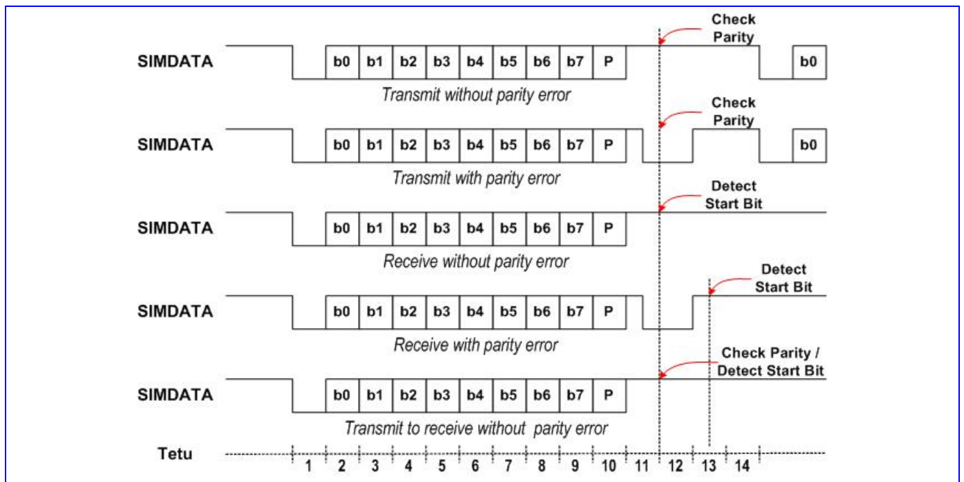
Figure 24 SIM Interface Timing Diagram
