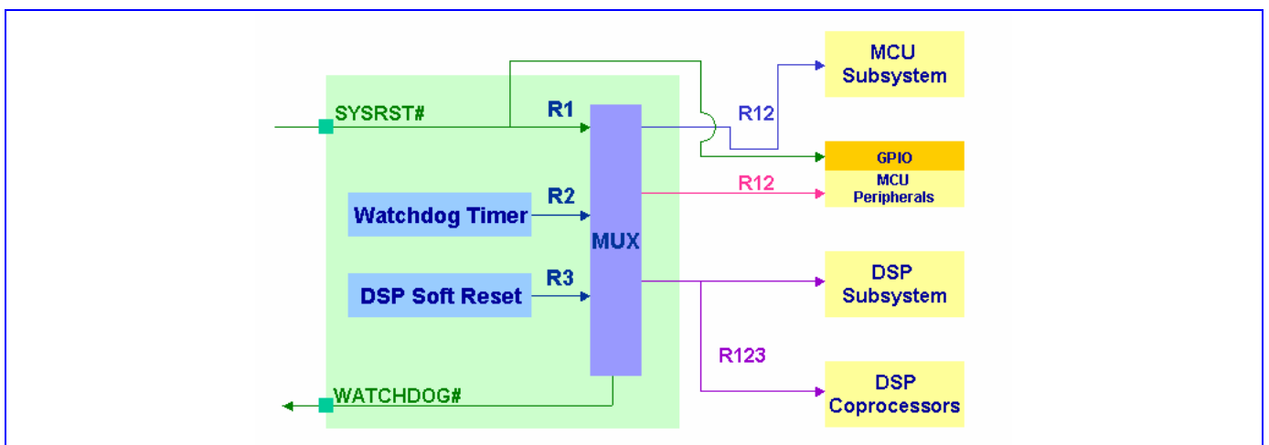
Figure 73 Reset Scheme Used in MT6223
