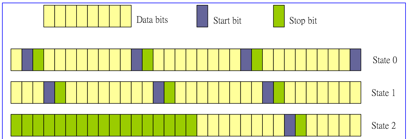
Figure 41 Example of Back to state 0
