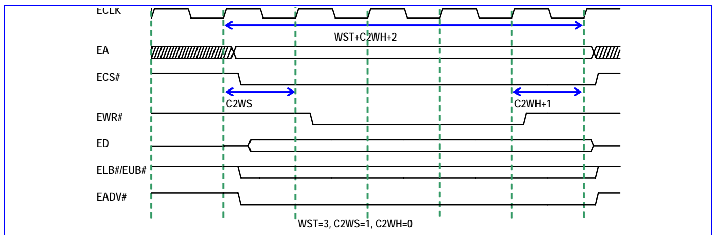
Figure 18 Write Wait State Timing Diagram (ADVW=1)
