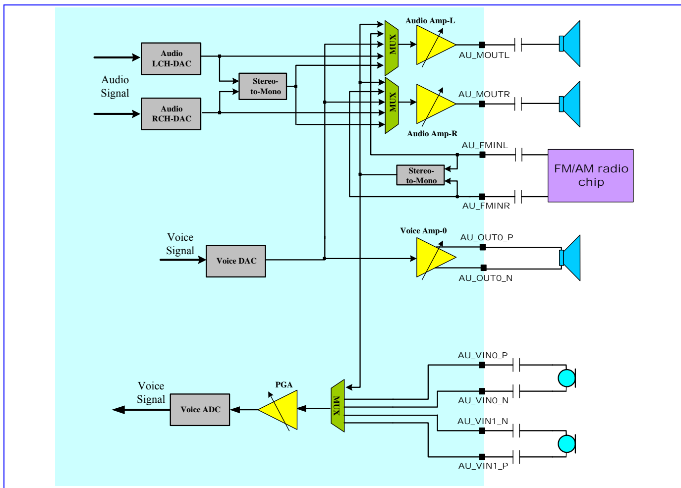
Figure 75 Block diagram of audio mixed-signal blocks.
