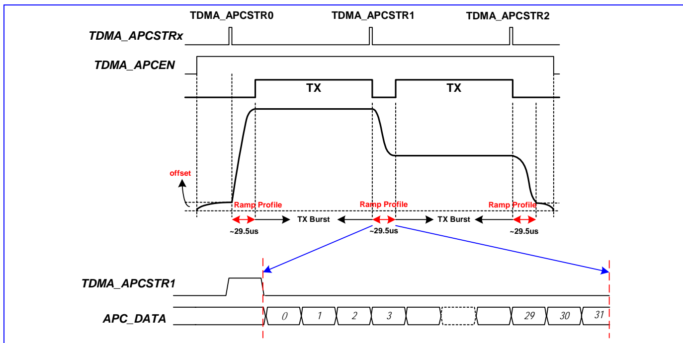
Figure 49 Timing diagram of the APC ramping.
