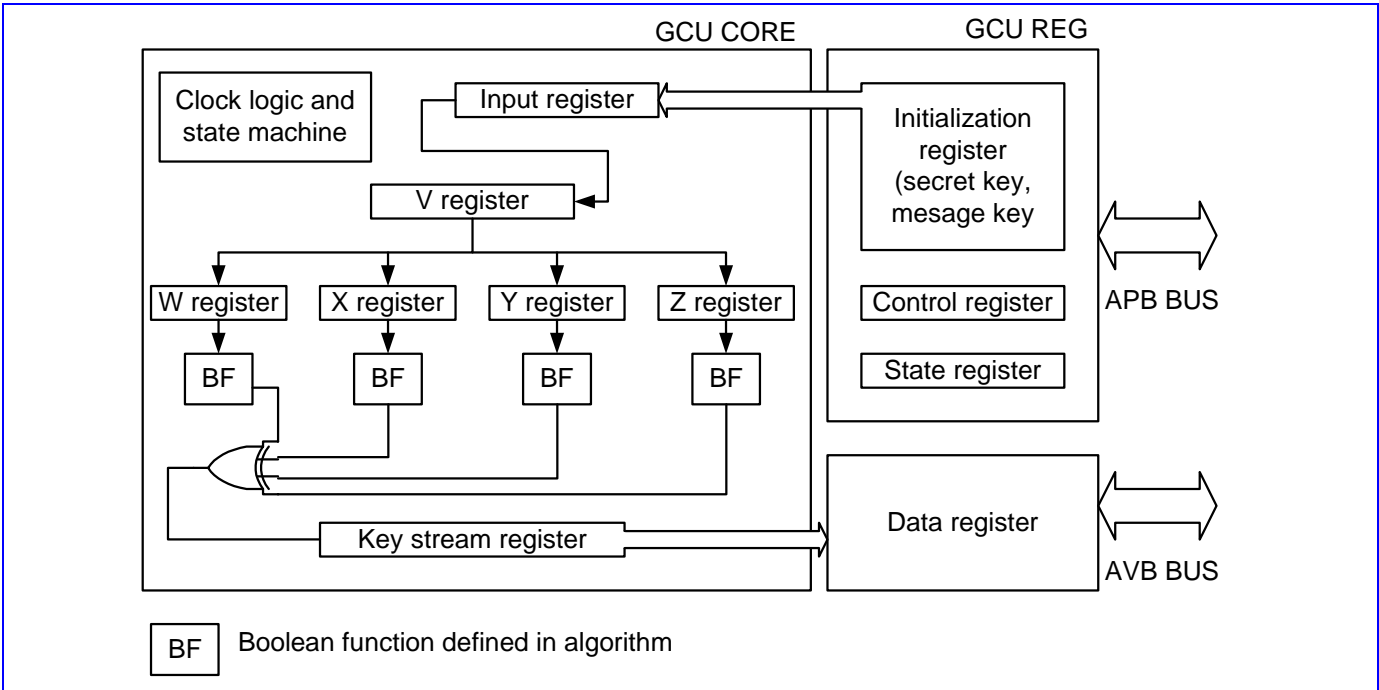
Figure 31 The block diagram of the GCU
