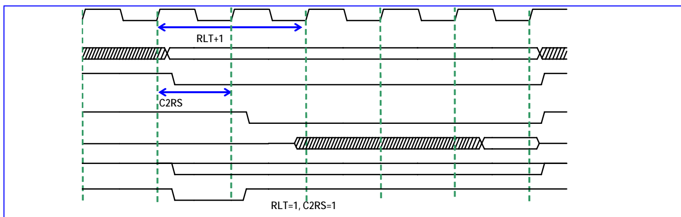
Figure 17 Read Wait State Timing Diagram (ADVR=0)
