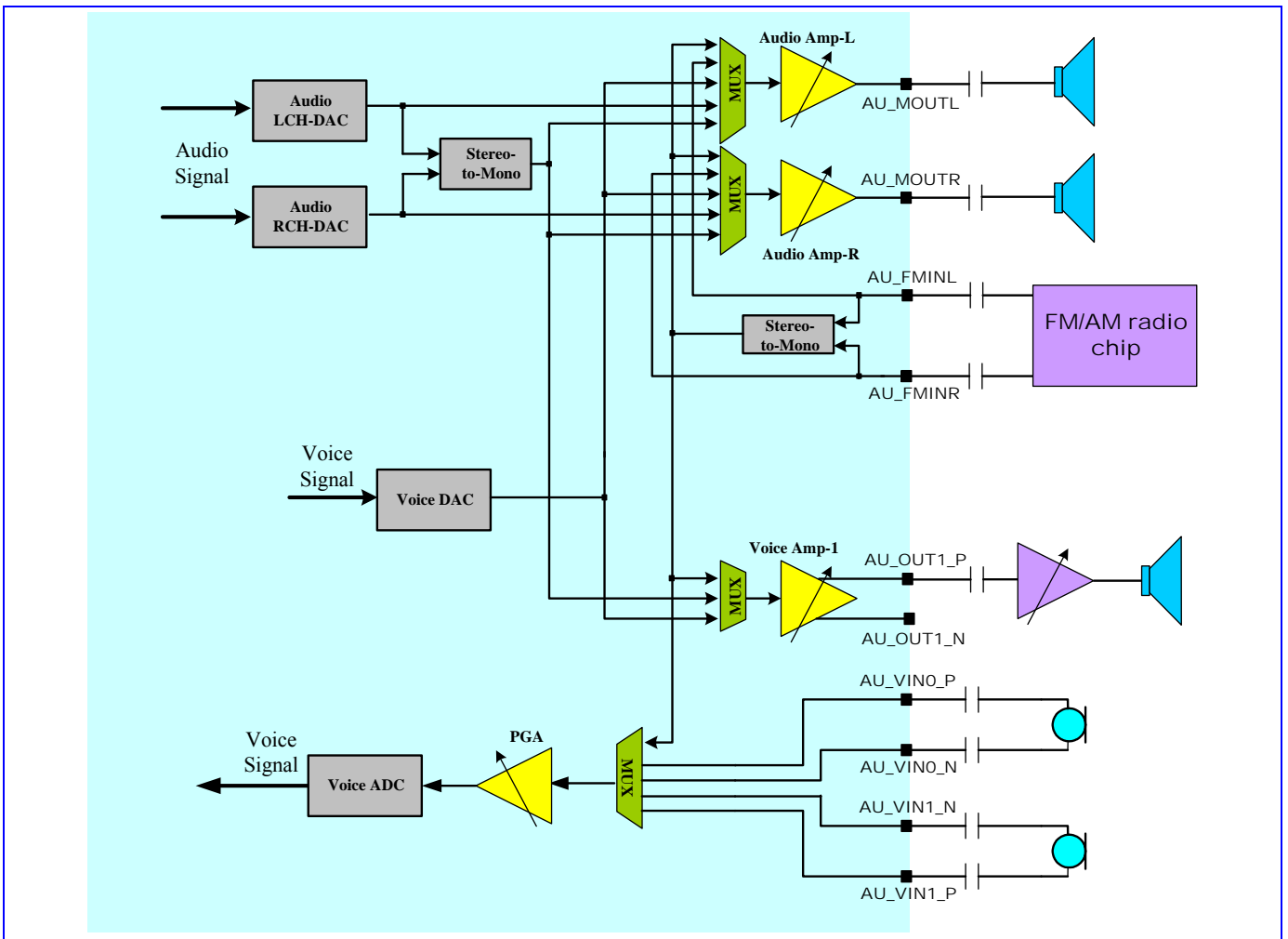
Figure 56 Block diagram of audio front-end
