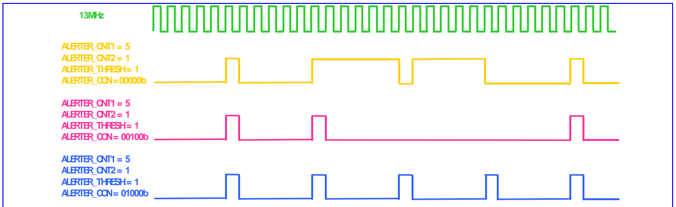
Figure 22 Alerter Output Signal from Enhanced PWM with Register Value Present
