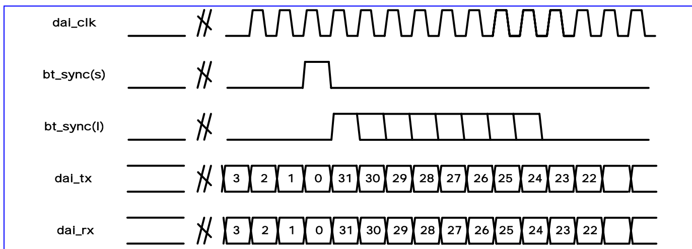
Figure 58 Timing diagram of Bluetooth application
