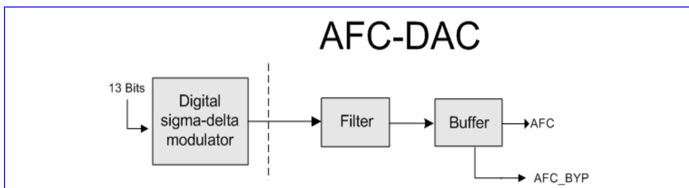
Figure 74 Block diagram of AFC-DAC
