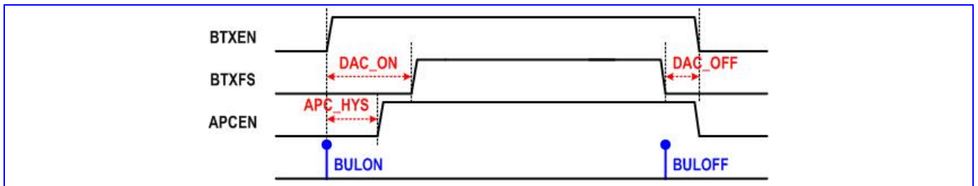
Figure 67 The timing diagram of BTXEN and BTXFS
