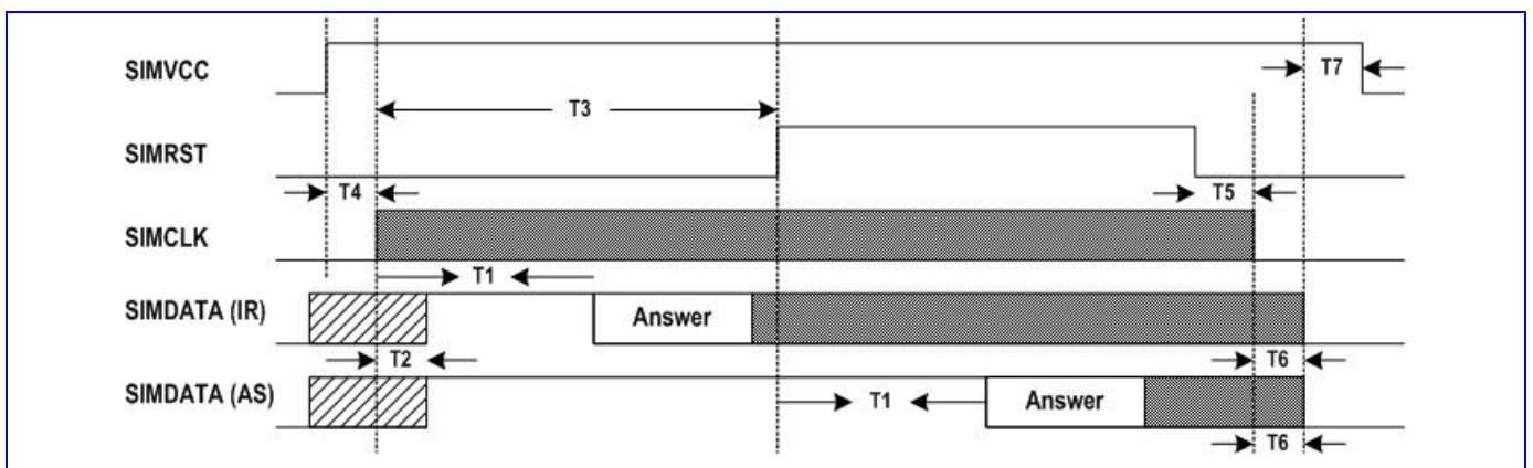
Figure 25 Answer to Reset Sequence
