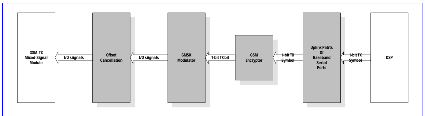
Figure 55 Block Diagram of Uplink Path
