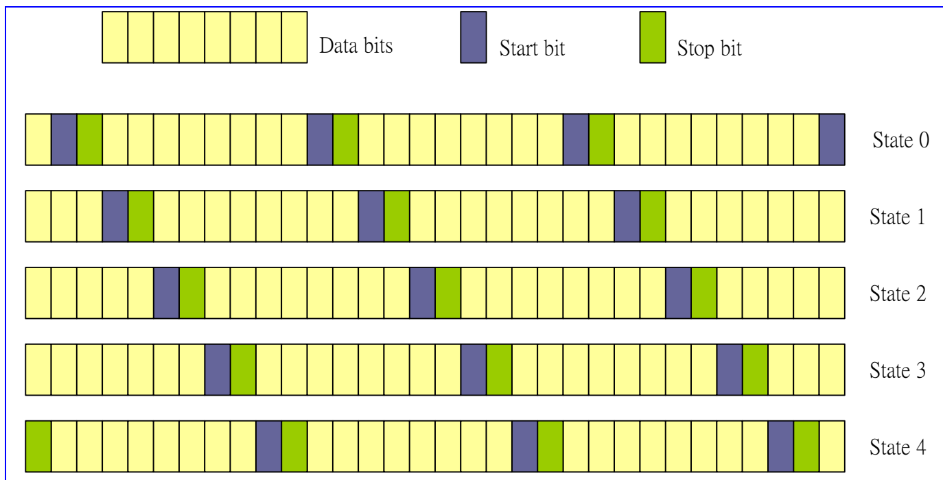
Figure 36 data format conversion of RA0
