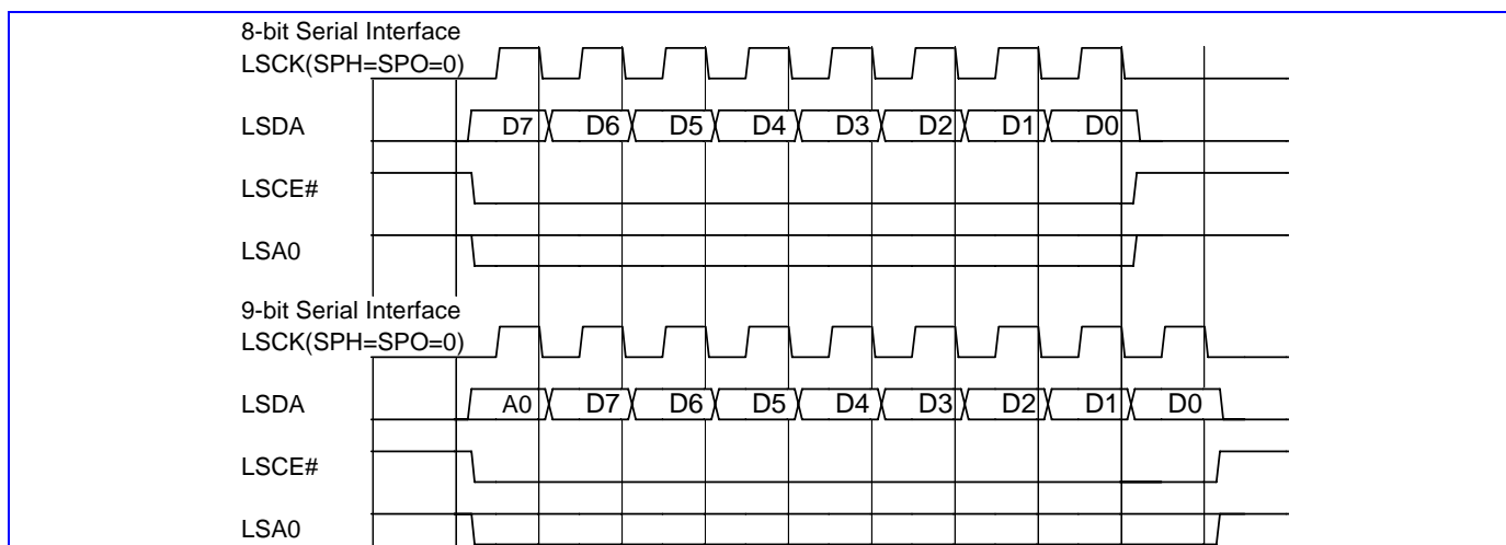
Figure 27 LCD Interface Transfer Timing Diagram
