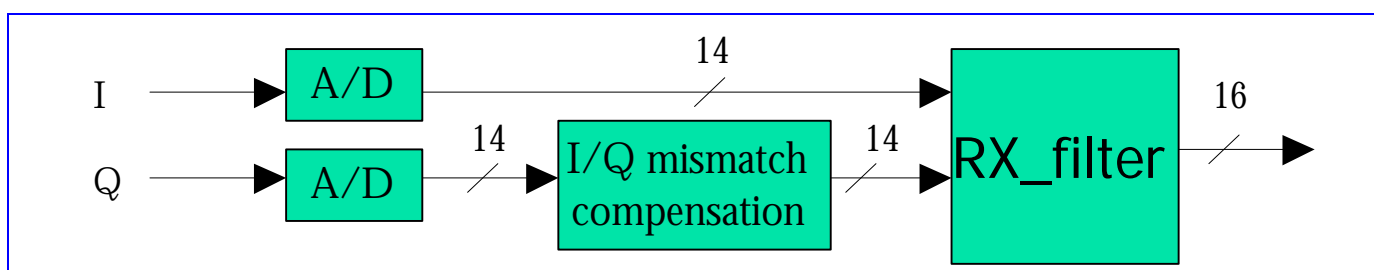
Figure 54 I/Q Mismatch Compensation Block Diagram
