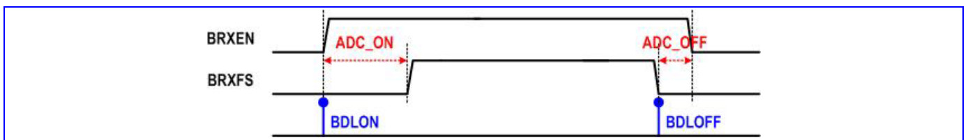
Figure 66 The timing diagram of BRXEN and BRXFS
