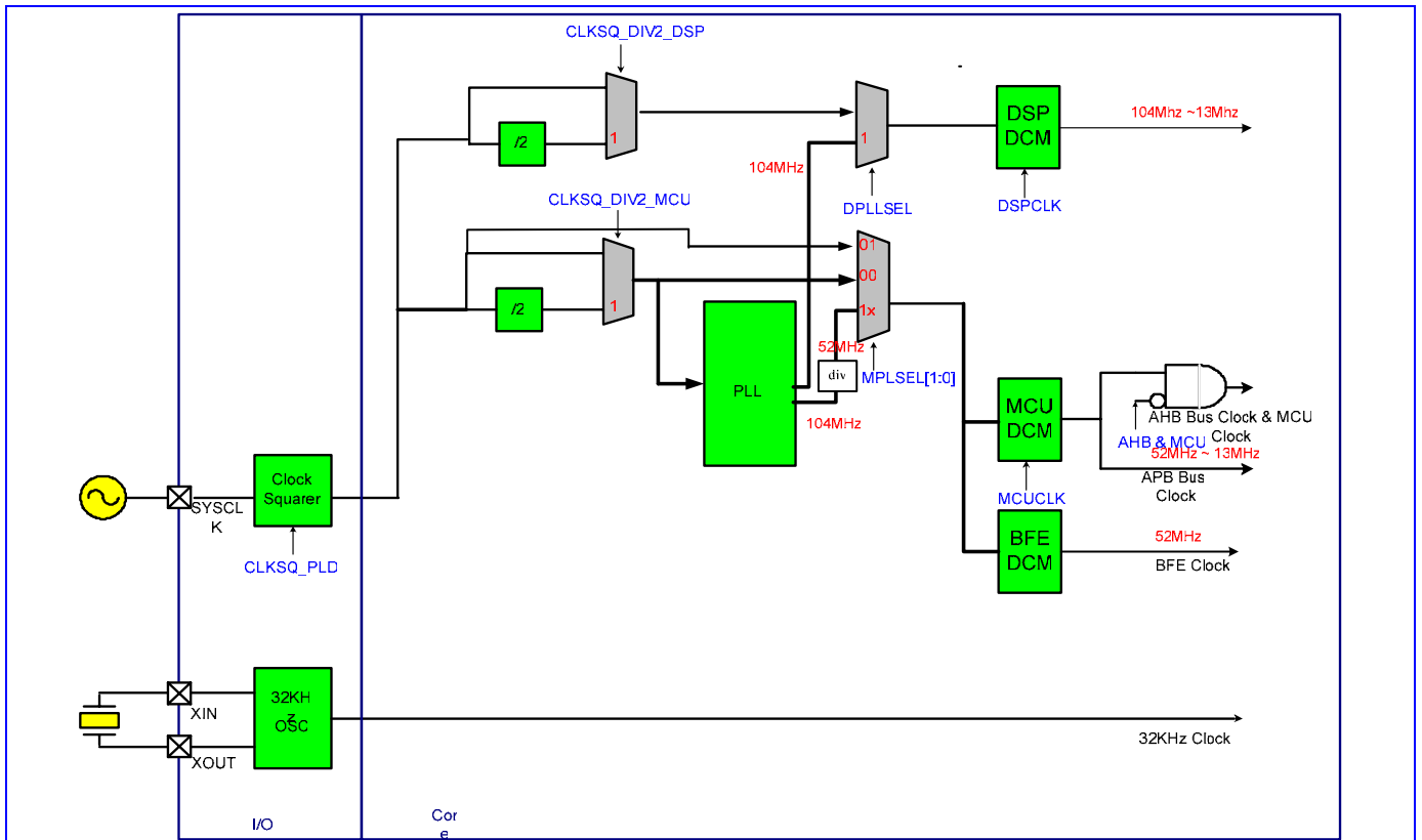
Figure 70 Clock distributions inside the MT6223.
