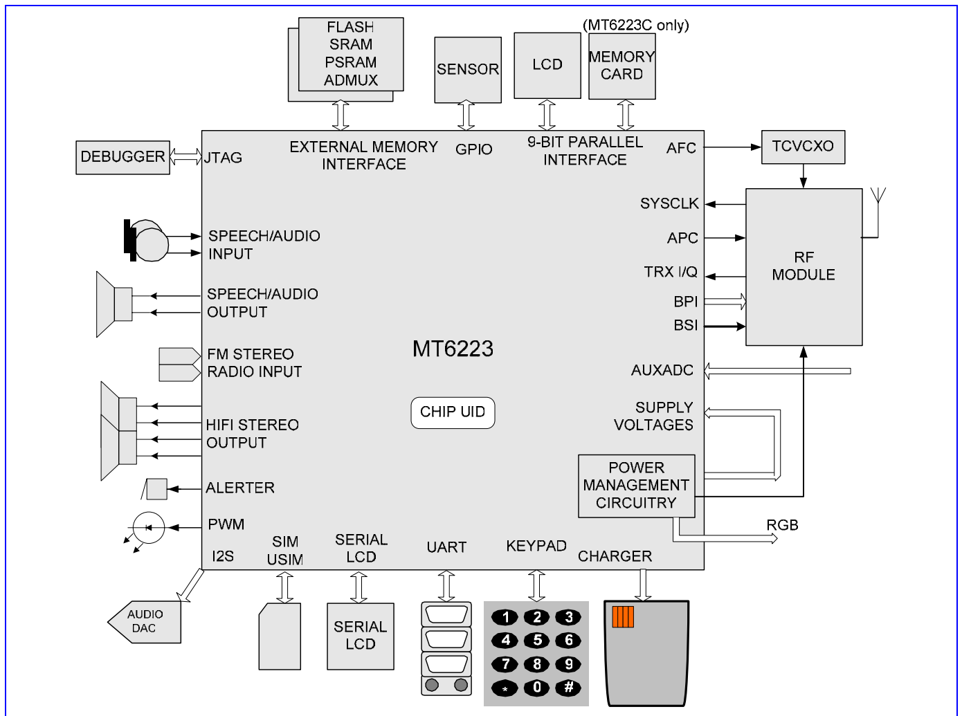
Figure 1 Typical application of MT6223.
