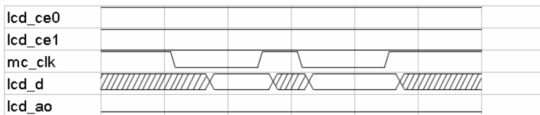
Figure 28 MSDC Interface Timing
