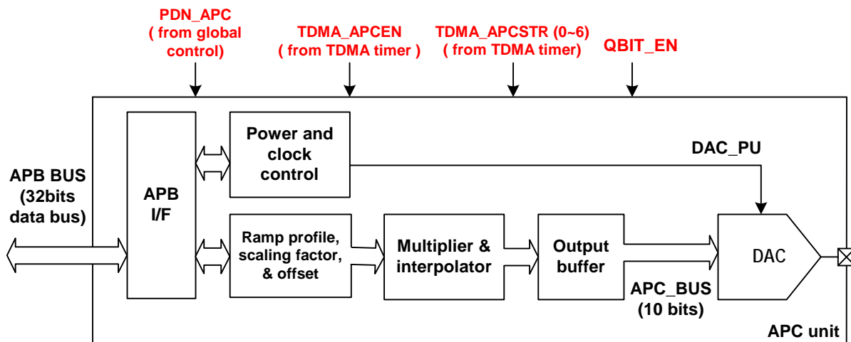
Figure 46 Block diagram of APC unit.
