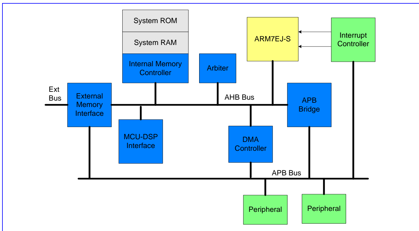
Figure 5 Block Diagram of the Micro-Controller Unit Subsystem in MT6223
