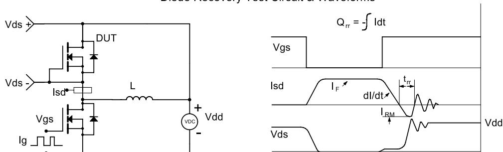
Diode Recovery Test Circuit &amp; Waveforms
