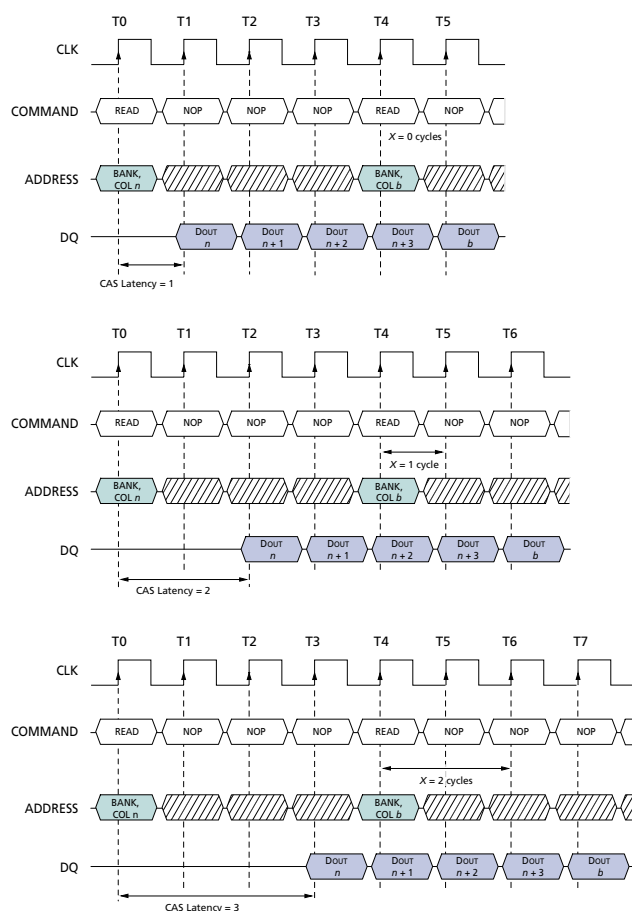
Figure 2 CAS Latency
