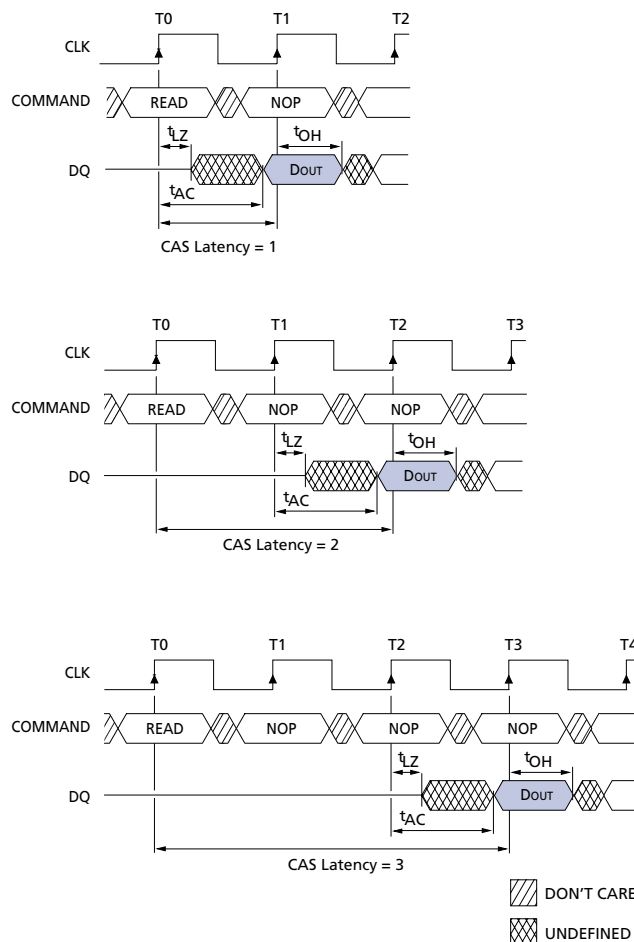
Figure 6 CAS Latency
