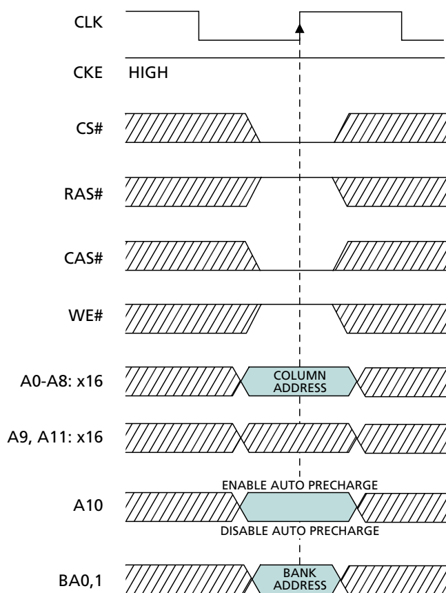
Figure 5 READ Command
