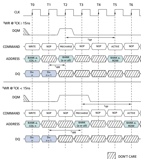
Figure 21: WRITE-To-PRECHARGE
