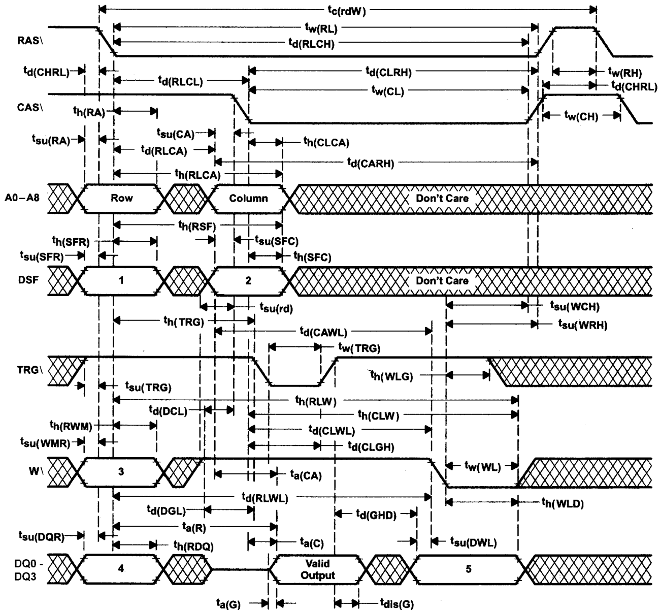
FIGURE 16: Read-Write/Read-Modify-Write-Cycle Timing
