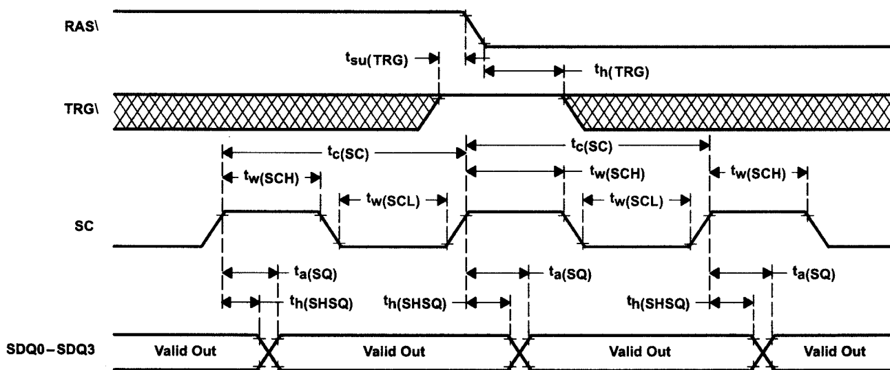
FIGURE 38: Serial-Read-Cycle Timing ( SE \setminus = V_{IL} )
