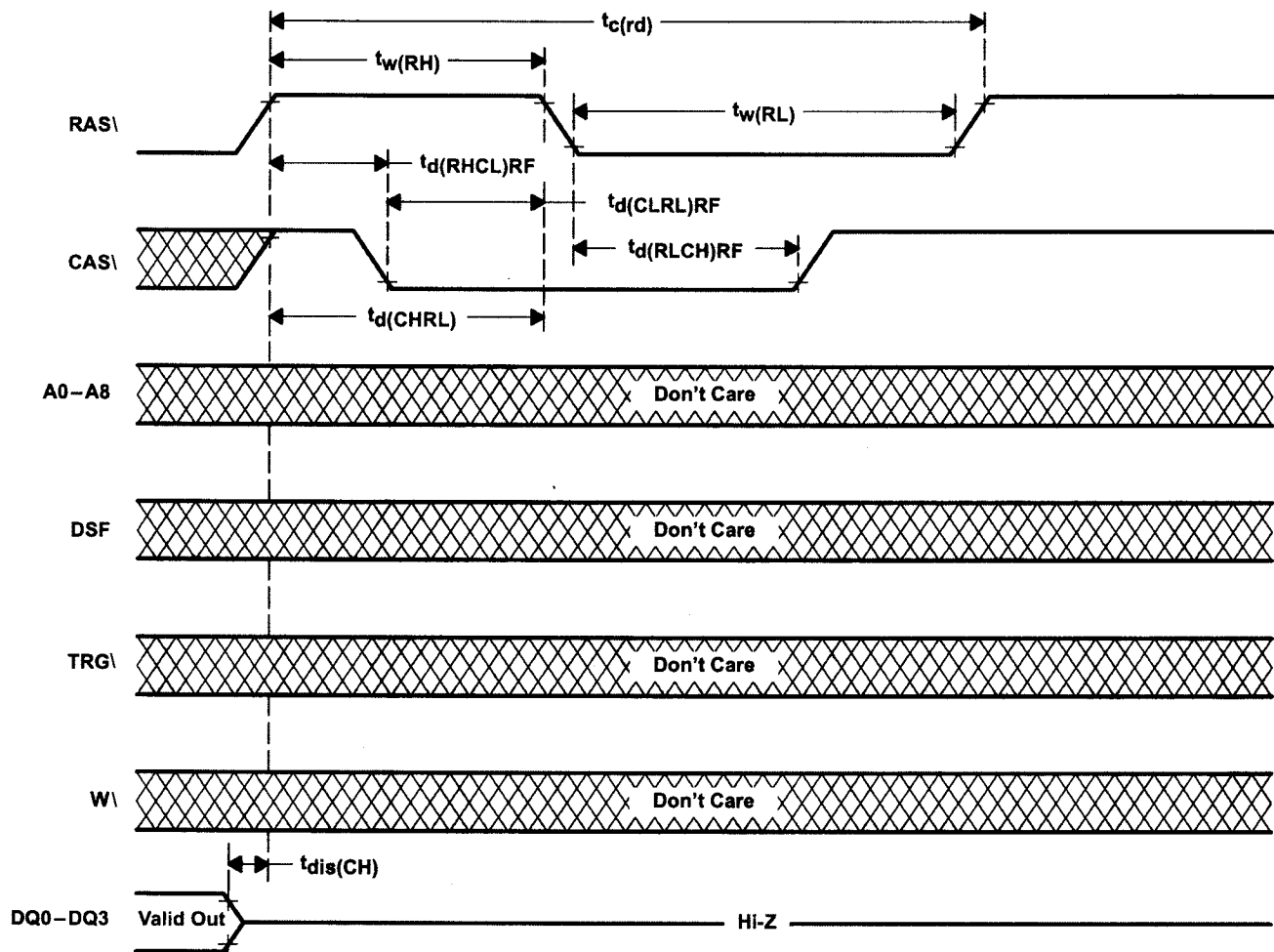
FIGURE 26: CBR-Refresh-Cycle Timing
