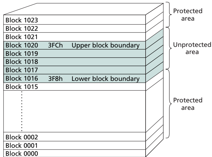
Figure 46: Flash Array Protected: Invert Area Bit = 0
