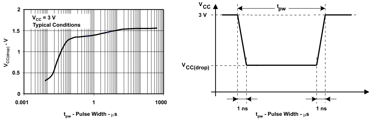
Figure 5-8. V_{CC(drop)} Level with a Square Voltage Drop to Generate a POR or BOR Signal
