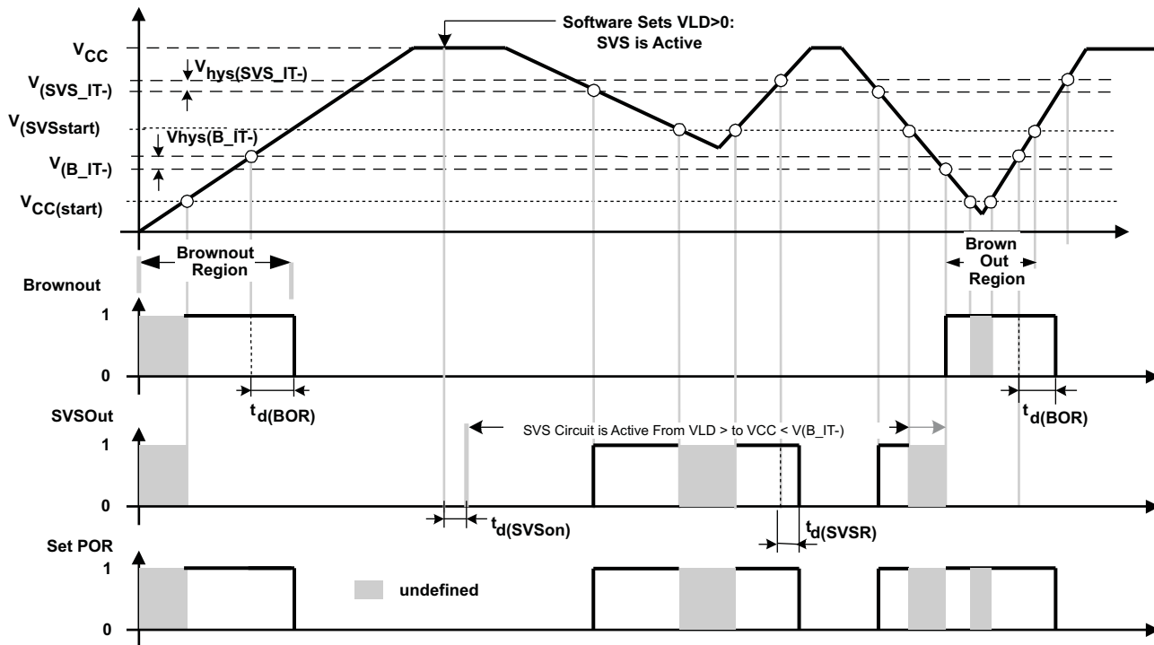
Figure 5-10. SVS Reset (SVSR) vs Supply Voltage
