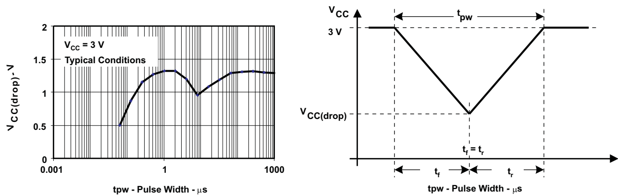
Figure 5-9. V_{CC(drop)} Level With a Triangle Voltage Drop to Generate a POR or BOR Signal
