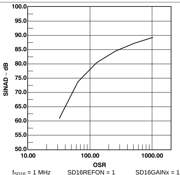
Figure 5-19. SINAD Performance vs OSR
