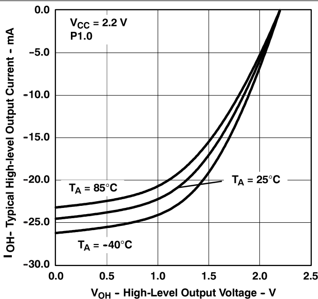
Figure 5-5. Typical High-Level Output Current vs Typical High-Level Output Current
