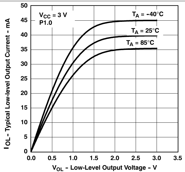
Figure 5-4. Typical Low-Level Output Current vs Typical Low-Level Output Current
