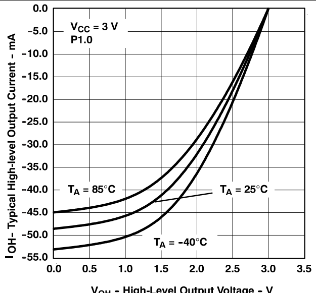
Figure 5-6. Typical High-Level Output Current vs Typical High-Level Output Current
