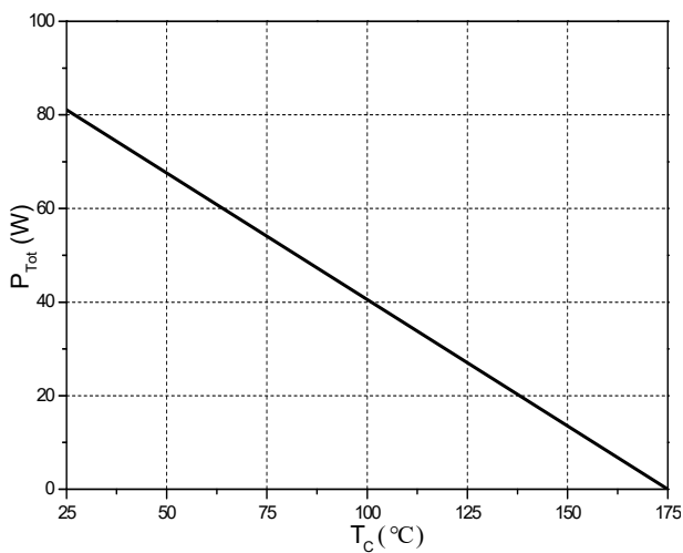
Figure 6. Power Derating
