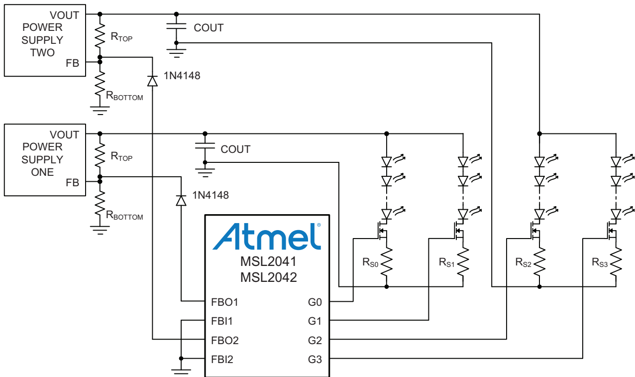
Figure 7-4. EO Configuration When Using Two String Power Supply.
