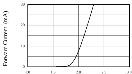
FIG.3 FORWARD CURRENT VS. FORWARD VOLTAGE
