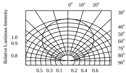
FIG.6 RADIATION PATTERN DIAGRAM
