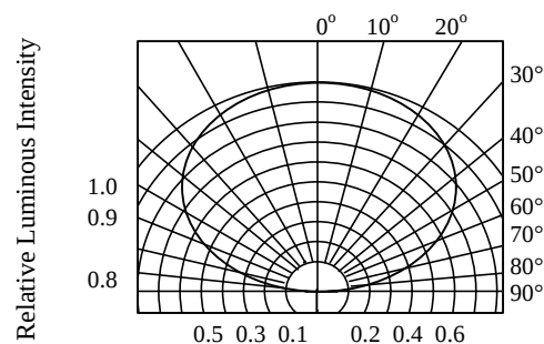
FIG.6 RADIATION DIAGRAM
