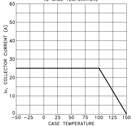
MAXIMUM CONTINUOUS COLLECTOR CURRENT vs CASE TEMPERATURE
