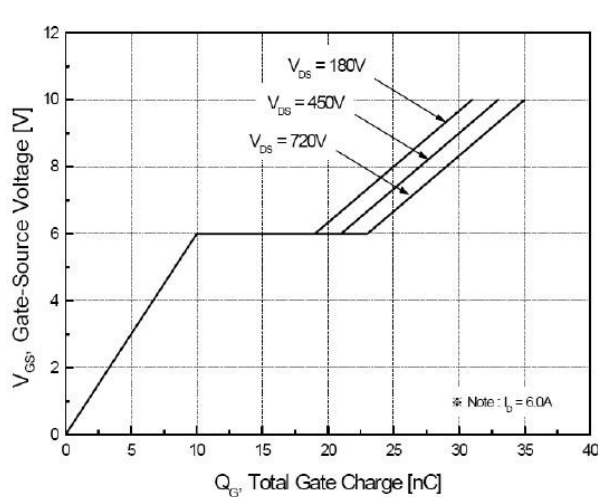
FIG.6-GATE CHARGE CHARACTERISTICS
