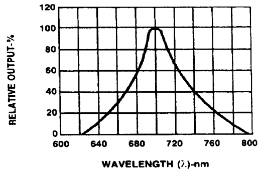
Fig.2 SPECTRAL RESPONSE
