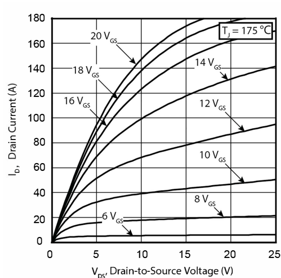
Figure 1-4. Drain Current vs. V_{DS} at V_{GS}
