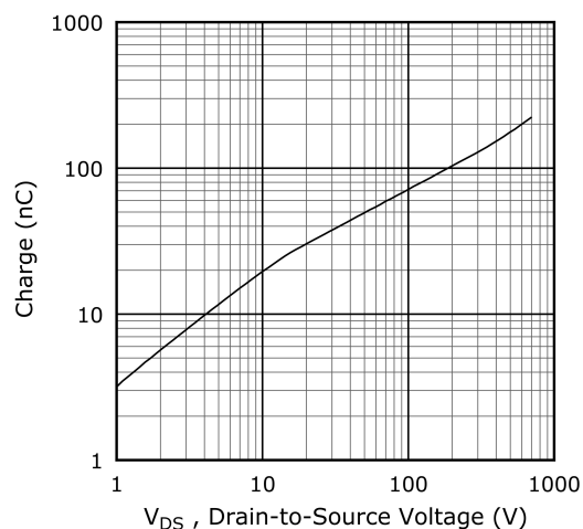
Figure 1-8. Output Charge vs. Drain-to-Source Voltage
