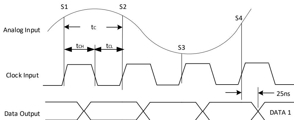
re 17. Timing Diagram
