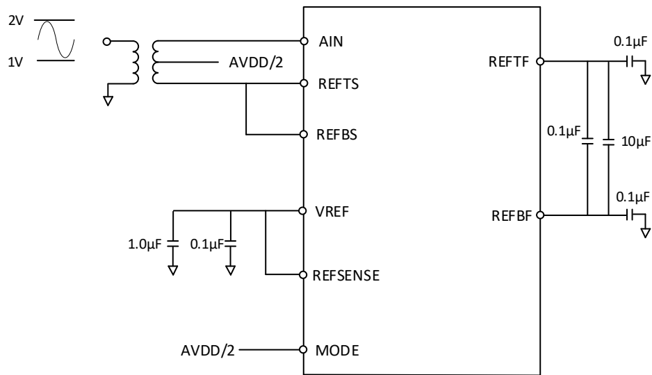
Figure 15. Differential Input Structure
