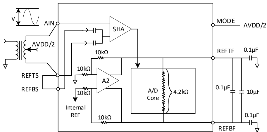
Figure 2c. Differential Mode
