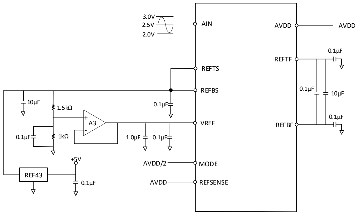
Figure 8. External Reference, 1V Input Range (Center Span Mode)
