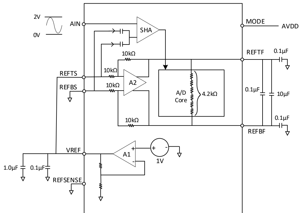
Figure 4. Internal Reference, 2V Input Range (Top/Bottom Mode)
