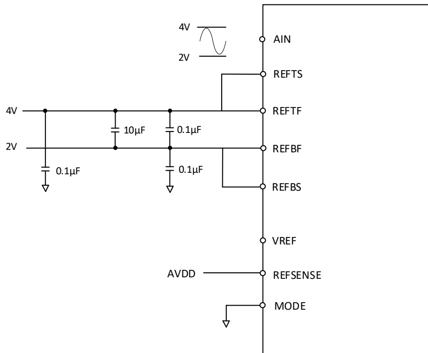
Figure 9a. External Reference, 2V Input Range (Top/Bottom Mode)
