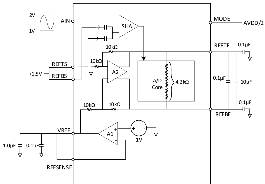
Figure 5. Internal Reference, 1V Input Range (Center Voltage Mode)
