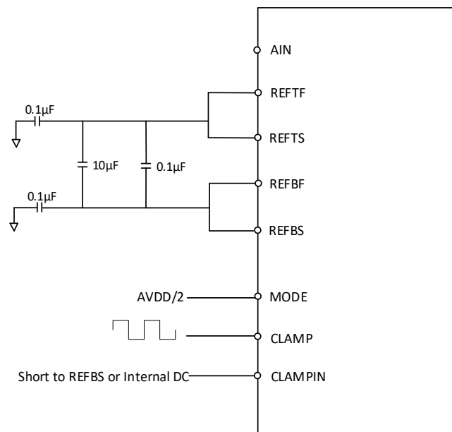
Figure 10b. Video Clamp Circuit
