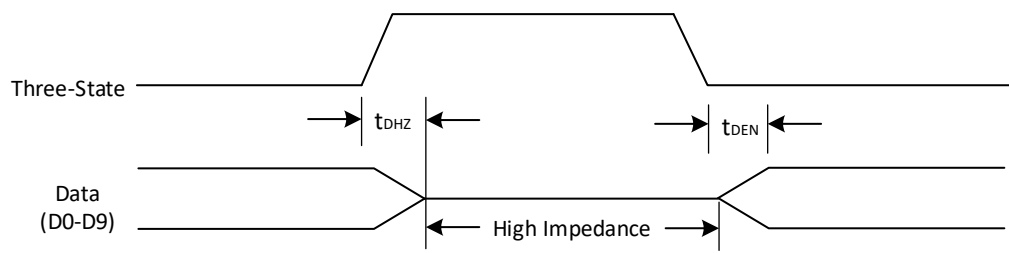
Figure 19. Three-State Timing Diagram
