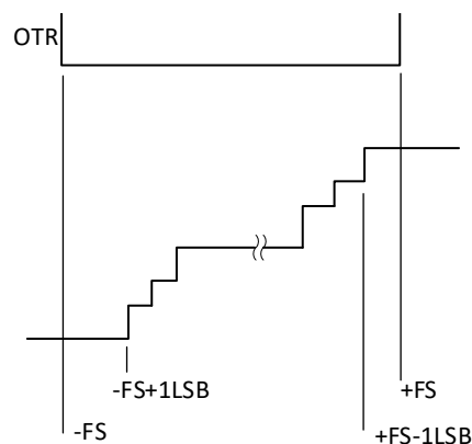
Figure 18. Data Output Format
