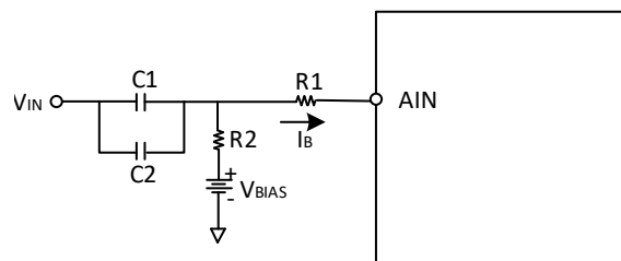
Figure 13. AC-Coupled Input
