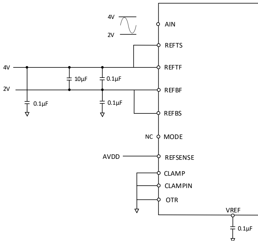
Figure 16. The AD876 Mode
