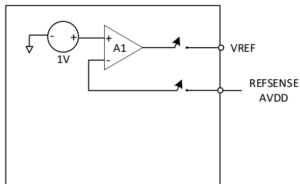
Figure 2g. Internal Reference Disable Mode
