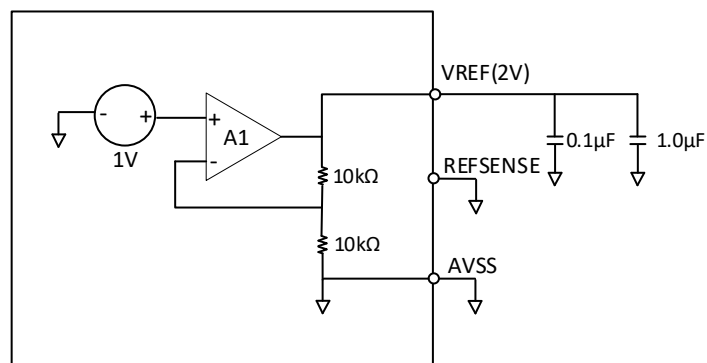
Figure 2e. 2V Reference Mode
