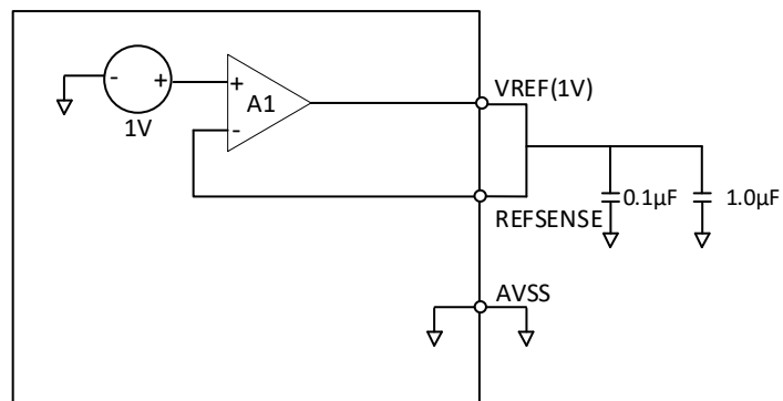
Figure 2d. 1V Reference Mode
