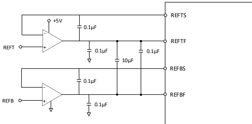
Figure 9b. Kelvin Connected External Reference Mode
