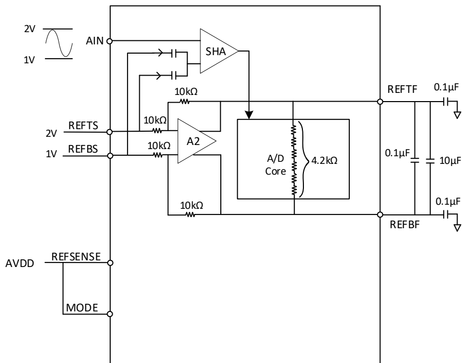
Figure 7. External Reference, 1V Input Range (Top/Bottom Mode)
