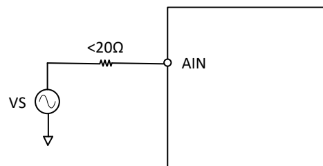
Figure 12. The MS9280 Simple Drive Circuit
