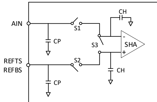
Figure 11. The MS9280 Equivalent Input Structure
