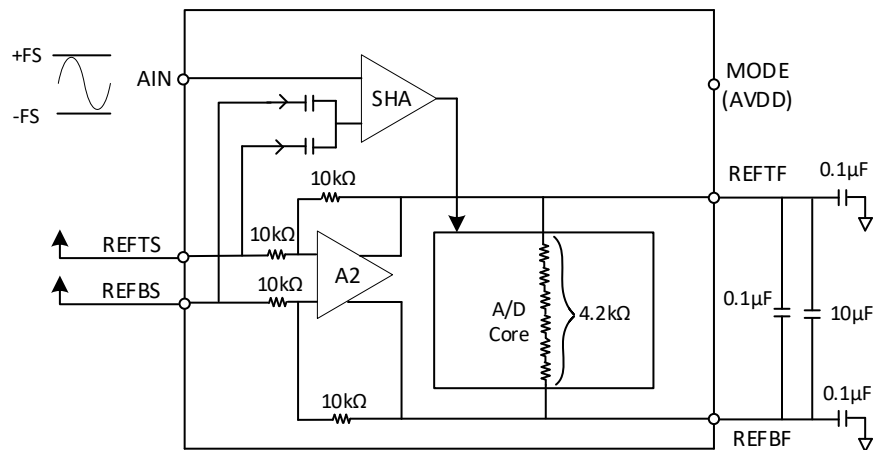
Figure 1. The MS9280 Equivalent Functional Input Circuit
