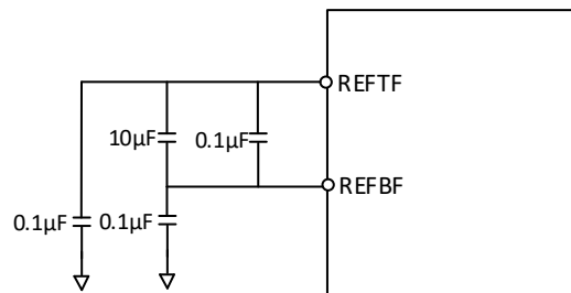
Figure 3. Reference Decoupling Network
