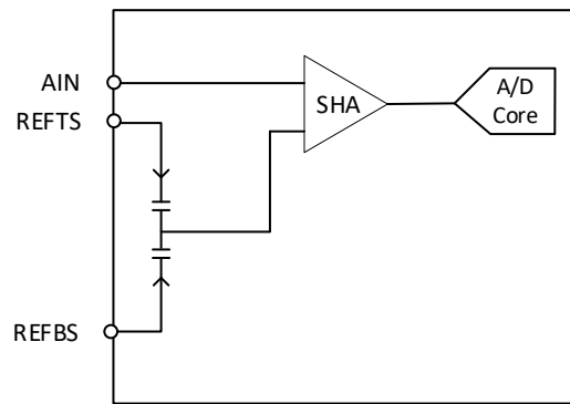
Figure 1. The MS9280 Equivalent Functional Input Circuit
