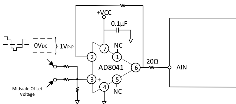
Figure 14. Bipolar Level Shift Structure
