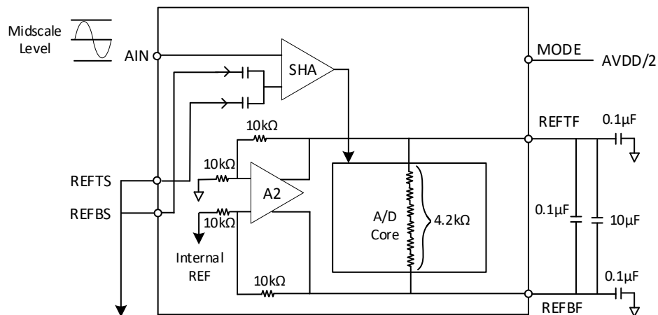
Figure 2b. Center Voltage Mode
