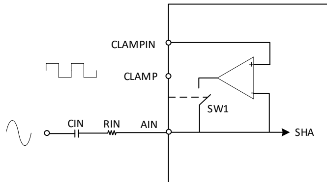
Figure 10a. Clamp Circuit
