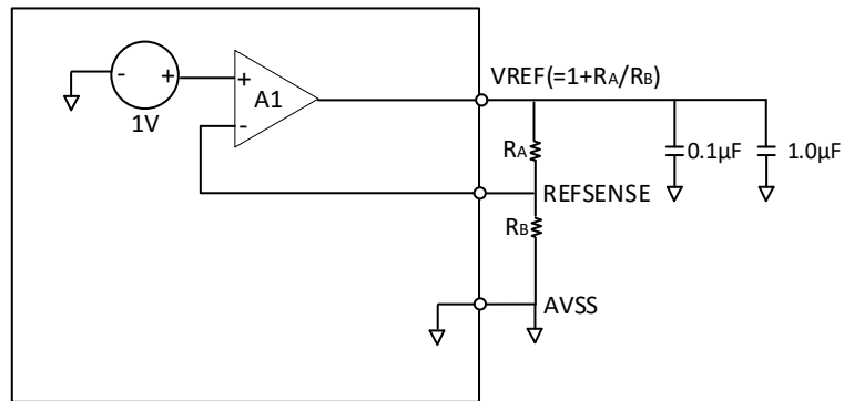
Figure 2f. Variable Reference Mode (between 1V and 2V)
