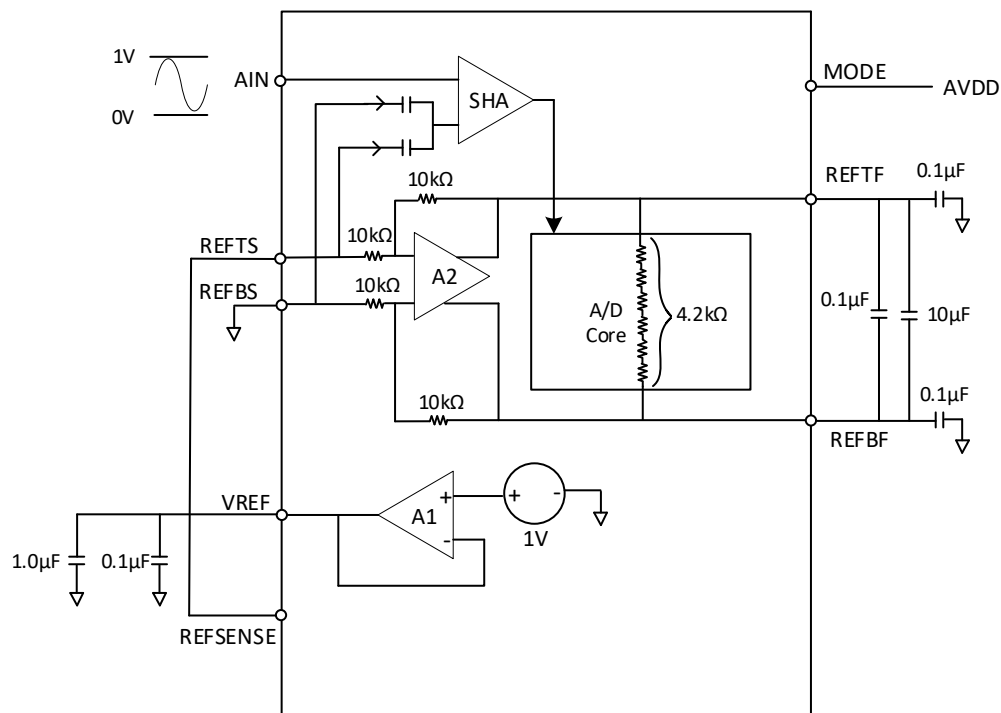
Figure 6. Internal Reference, 1V Input Range (Top/Bottom Mode)
