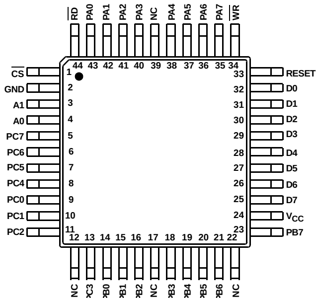
MQ82C55A (MQFP) TOP VIEW
