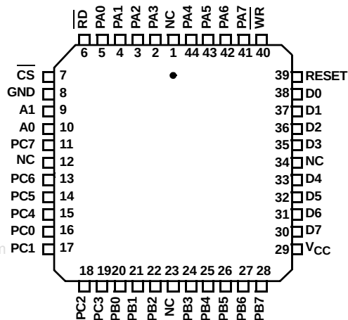
MS82C55A (PLCC) TOP VIEW
