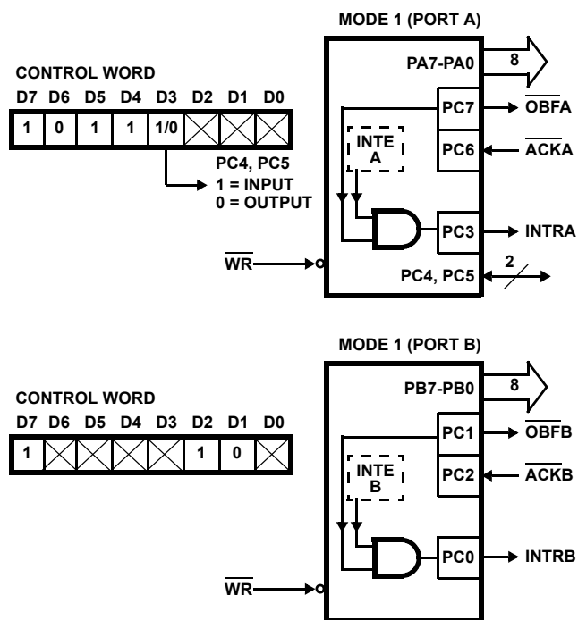
FIGURE 8. MODE 1 OUTPUT
