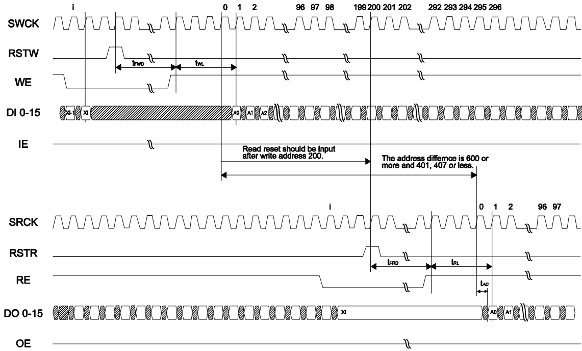
Read/Write Cycle Timing (New Data Read)
