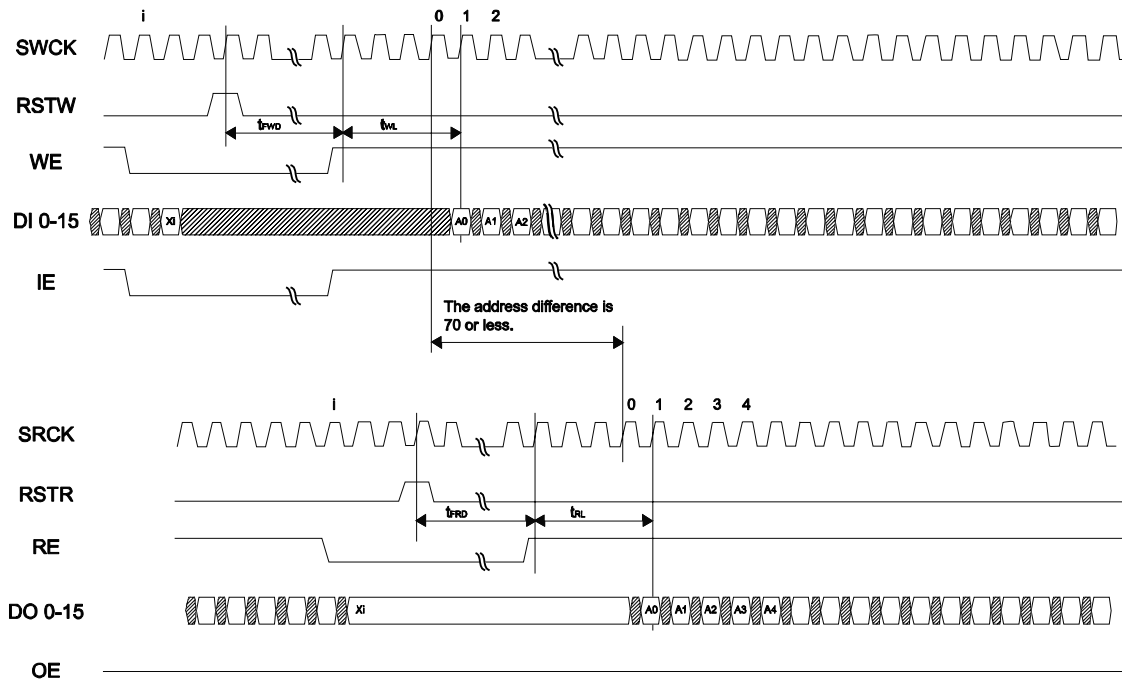
Read/Write Cycle Timing (Old Data Read)
