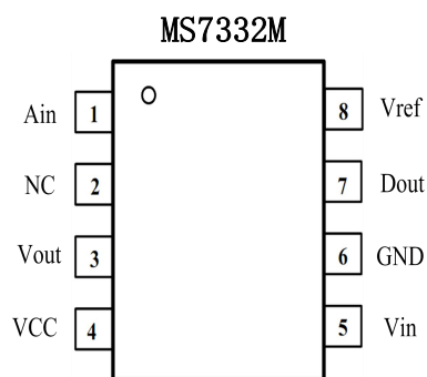
Figure1.MSOP-8
