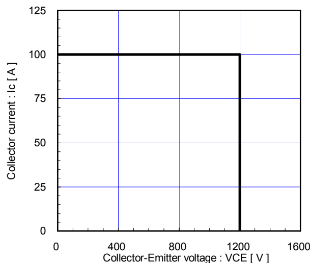
Reverse bias safe operating area (max.) +V_{GE}=15V , -V_{GE} \leq 15V , R_G \geq 22\Omega , T_J \leq 125^\circ C
