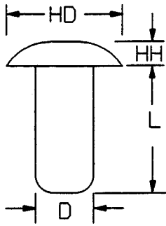
Universal Head
