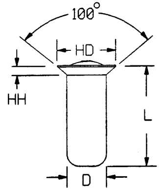
Reduced Countersunk Head
