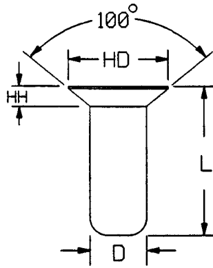
Countersunk Head
