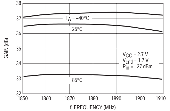
Figure 3. Gain versus Frequency (High Current Mode)
