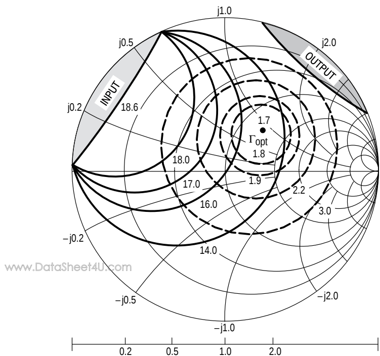
Figure 13. Constant Gain and Noise Figure Contours
