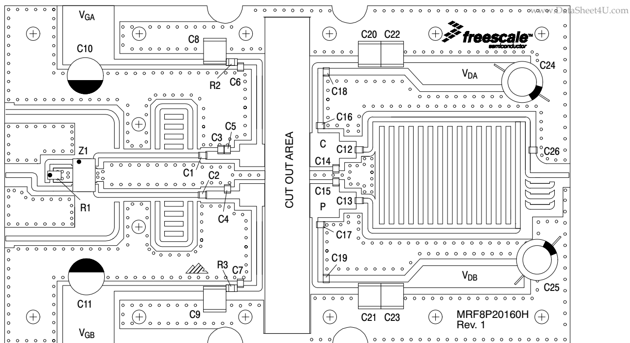
Figure 2. MRF8P20160HSR3 Test Circuit Component Layout
