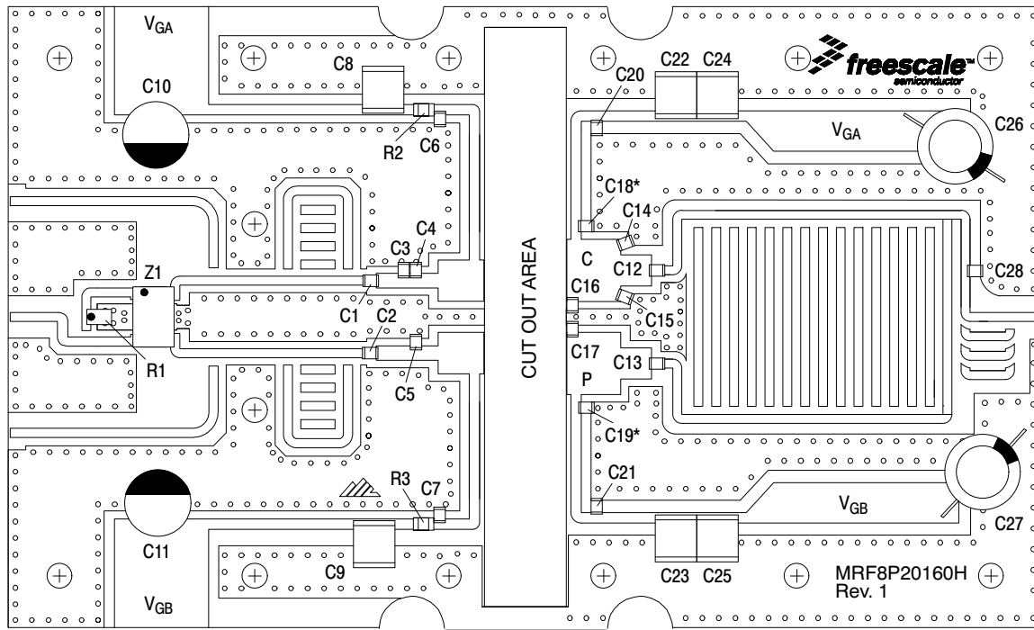
Figure 14. MRF8P20160HSR3 Test Circuit Component Layout — 2025 MHz
