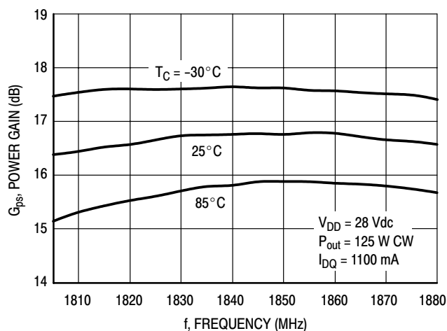
Figure 14. Power Gain versus Frequency
