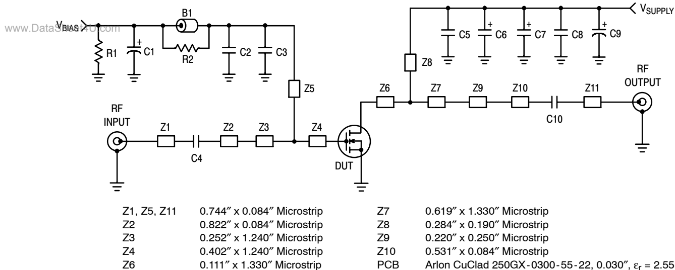
Figure 1. MRF7S16150HR3(HSR3) Test Circuit Schematic
