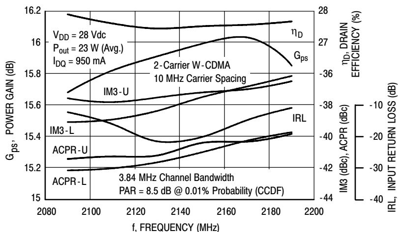
Figure 3. 2-Carrier W-CDMA Broadband Performance @ P_{out} = 23 Watts Avg.
