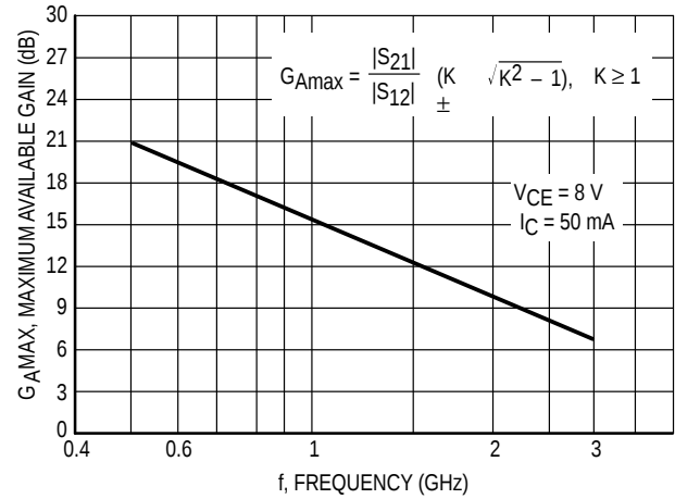
Figure 27. G_{Amax} , Maximum Available Gain versus Frequency
