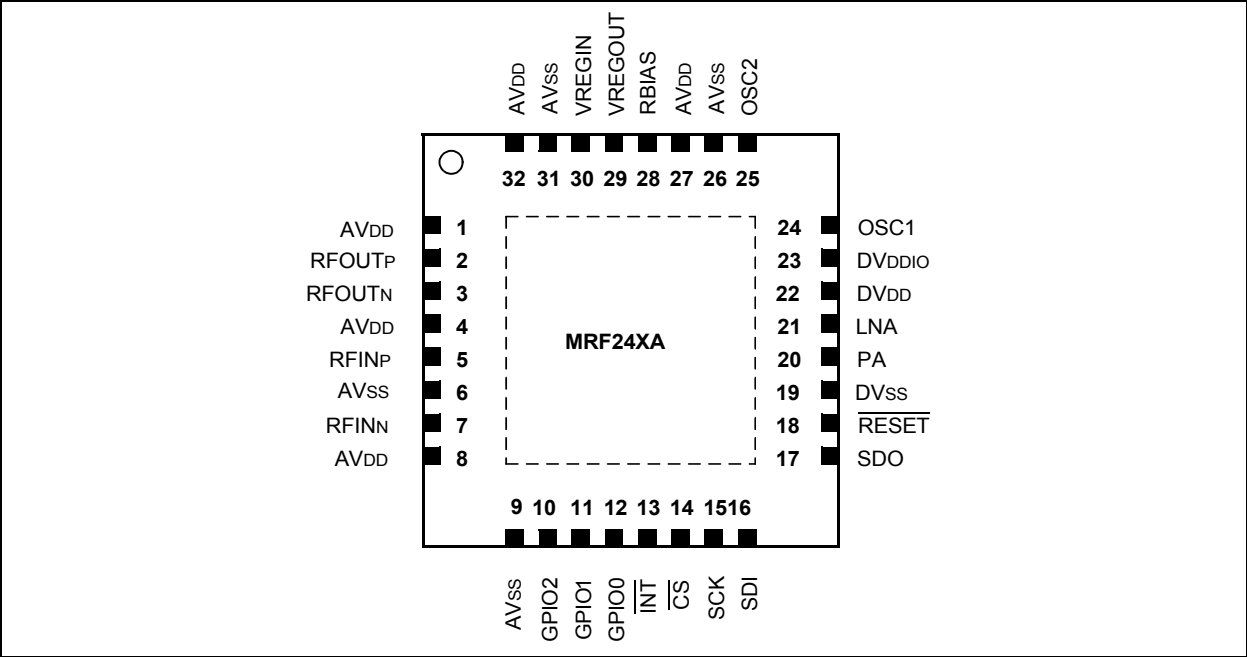
Pin Diagram
