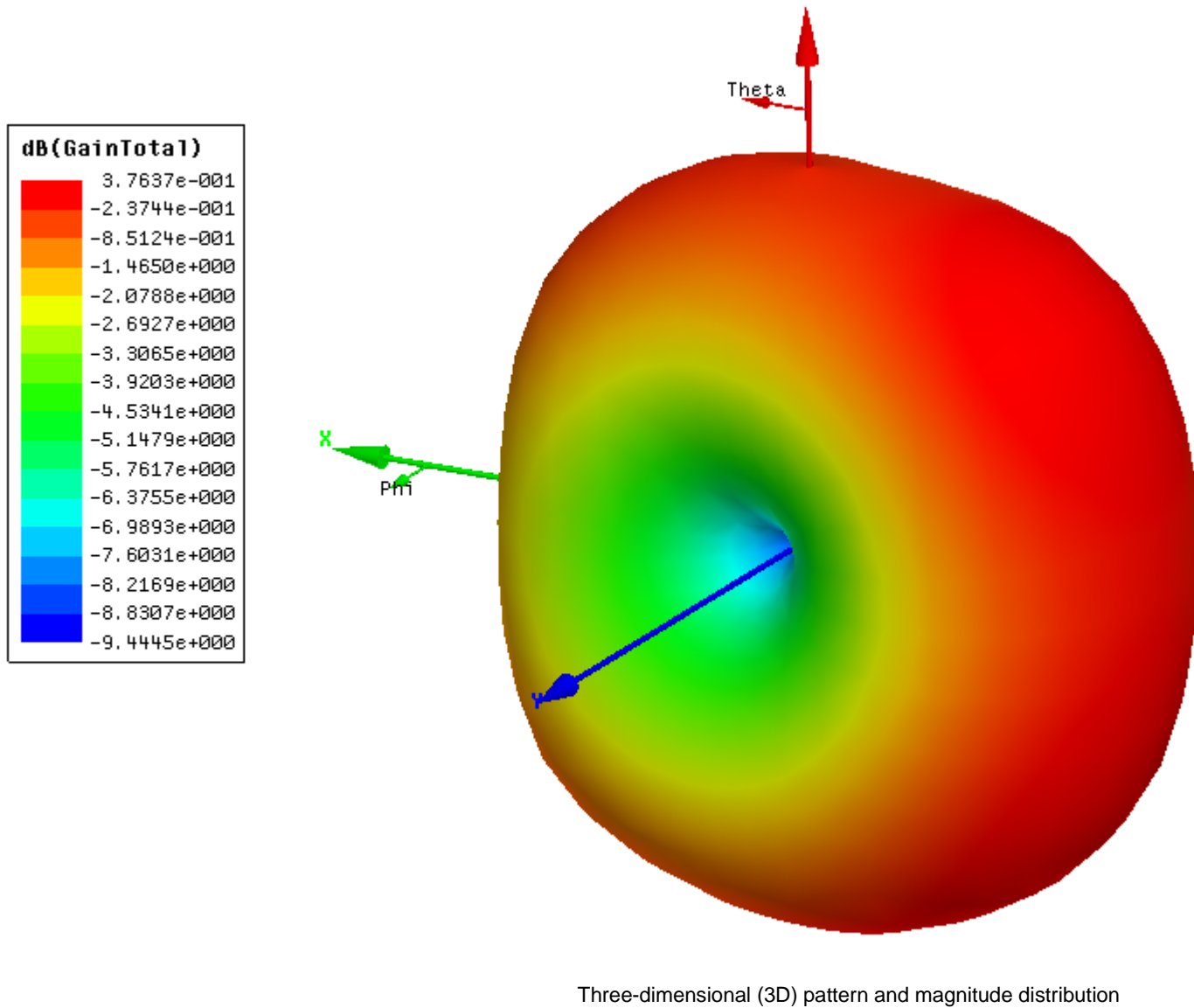
FIGURE 2-7: SIMULATED THREE-DIMENSIONAL RADIATION PATTERN
