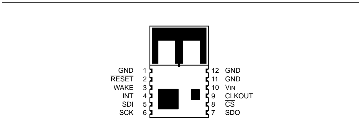
FIGURE 1: PIN DIAGRAM
