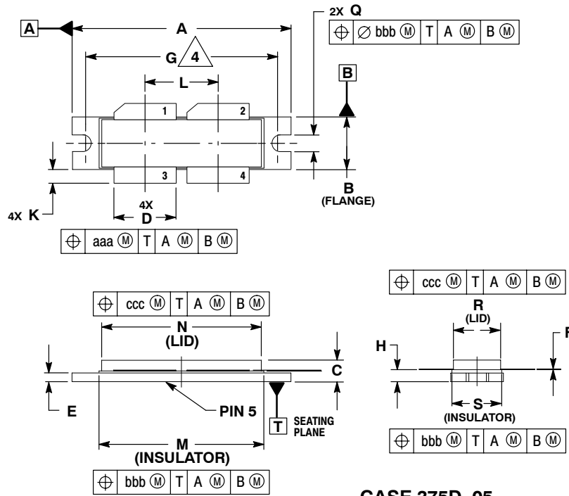
CASE 375D-05 ISSUE E NI-1230
