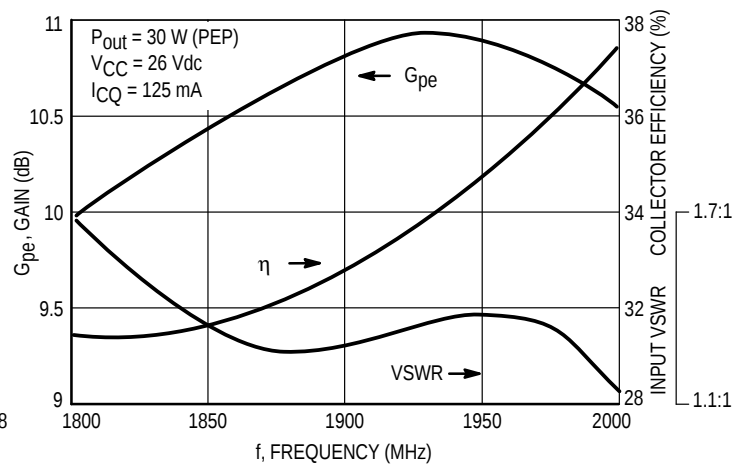
Figure 10. Performance in Broadband Circuit
