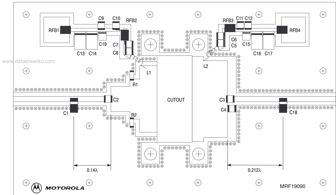
Figure 2. MRF19090 Test Circuit Component Layout
