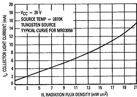
Figure 1. Collector Light Current
