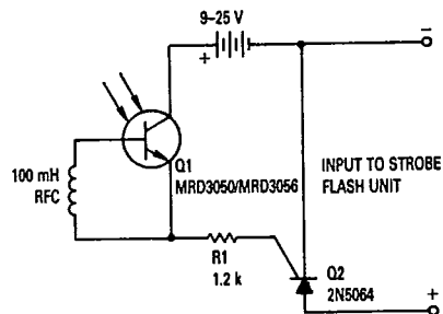
Figure 6. Strobe Flash Slave Adapter
