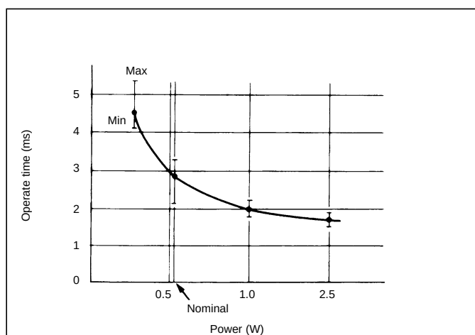
Operate Time
