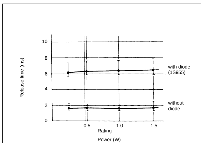
Release Time
