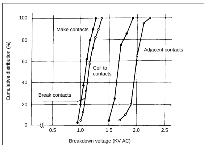
Breakdown Voltage
