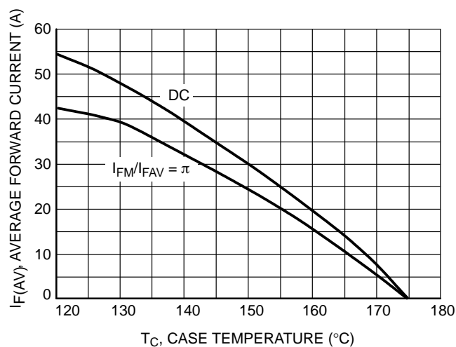
Figure 4. Current Derating
