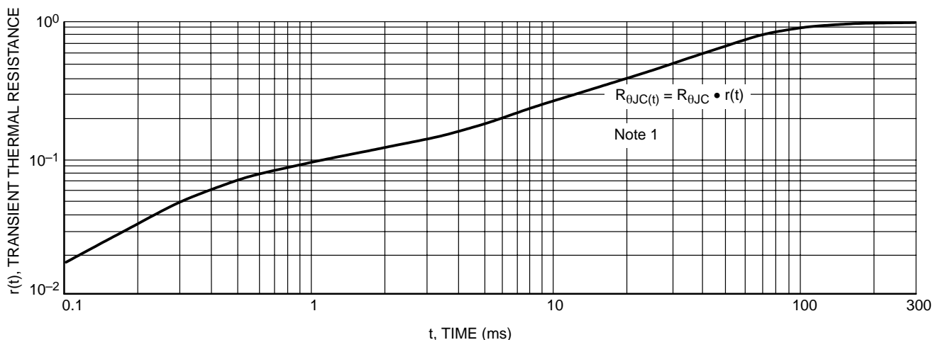
Figure 6. Thermal Response
