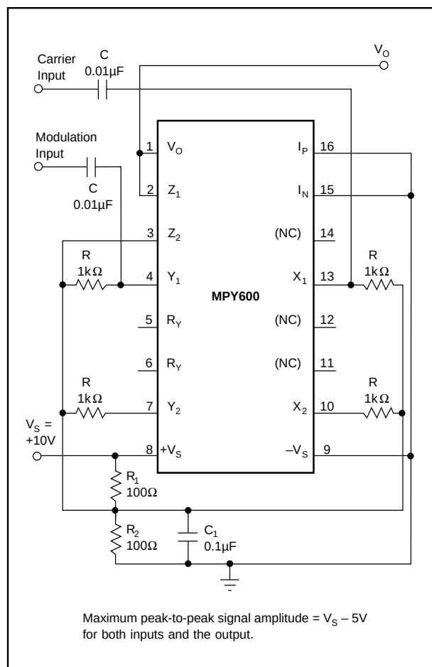
FIGURE 13. Single-Supply Balanced Modulator.
