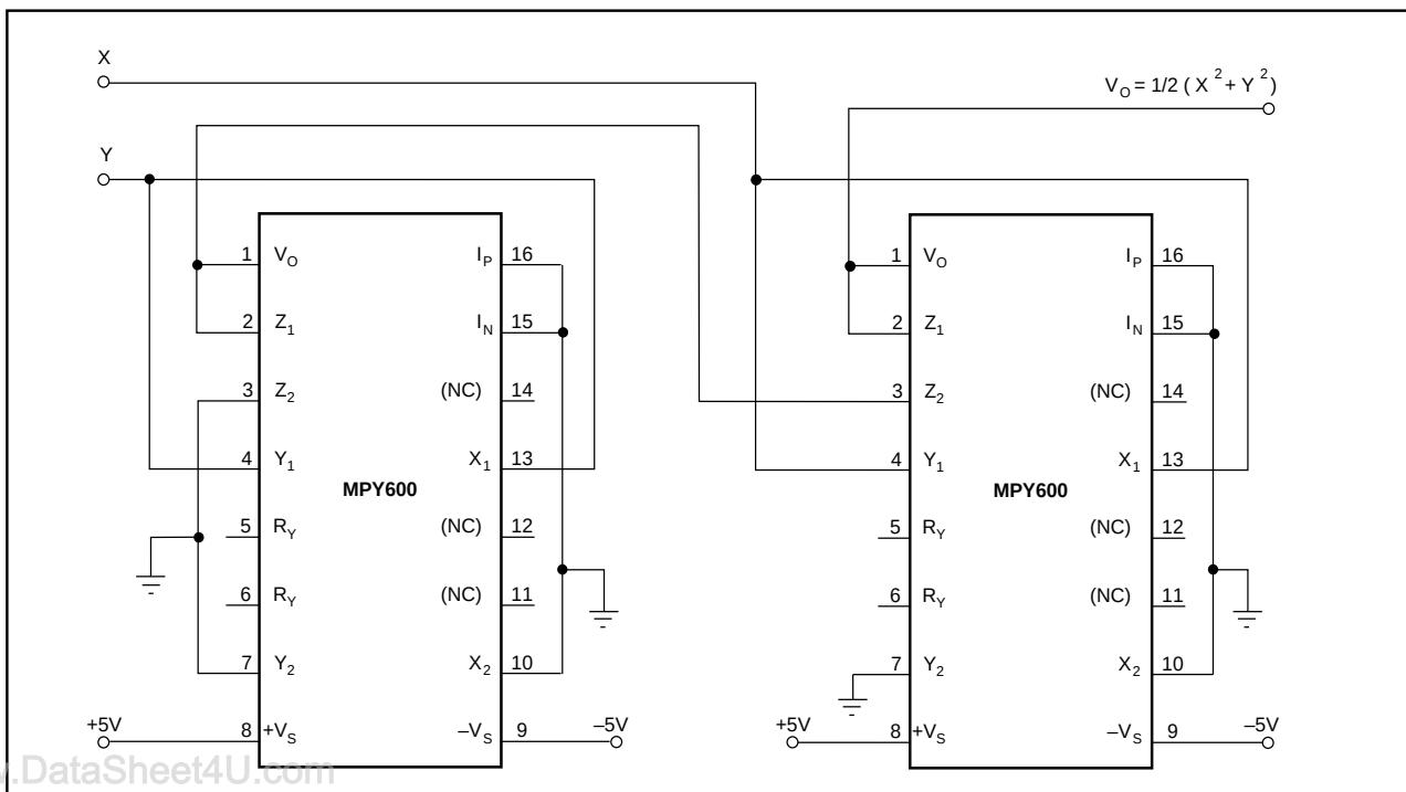
FIGURE 14. CRT Focus Correction.
