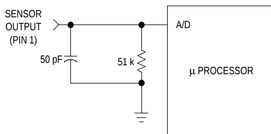
Figure 3. Decoupling Filter for Sensor to Microprocessor Interface
